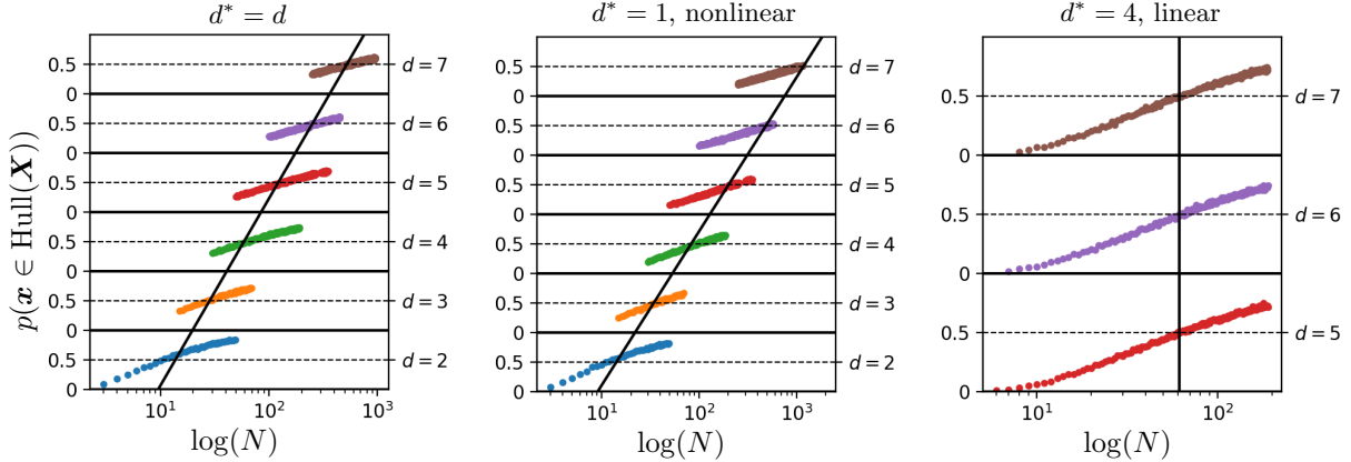
Figure 1: Depiction of the evolution of the probability that a new sample is in interpolation regime (y-axis, p(\mathbf{x} \in \text{Hull}(\mathbf{X})) ) given increasing dataset size (x-axis, N ) seen in logarithmic scale, and for various ambient space dimensions ( d ) based on Monte-Carlo estimates on 500,000 trials. On the left , the data is sampled from a Gaussian density \mathbf{x}_i \sim \mathcal{N}(0, I_d) while in the middle , the data is sampled from a nonlinear continuous manifold with intrinsic dimension of 1 (see Fig. 2 for details on the manifold data) and on the right , the data is sampled from a Gaussian density that lives in an affine subspace of constant dimension 4 (while the ambient dimension increases). It is clear from those figures that in order to maintain a constant probability to be in interpolation regime, the training set size has to increase exponentially with d^* regardless of the underlying intrinsic manifold dimension where d^* is the dimension of the lowest dimensional affine subspace including the entire data manifold i.e. the convex hull dimension.
