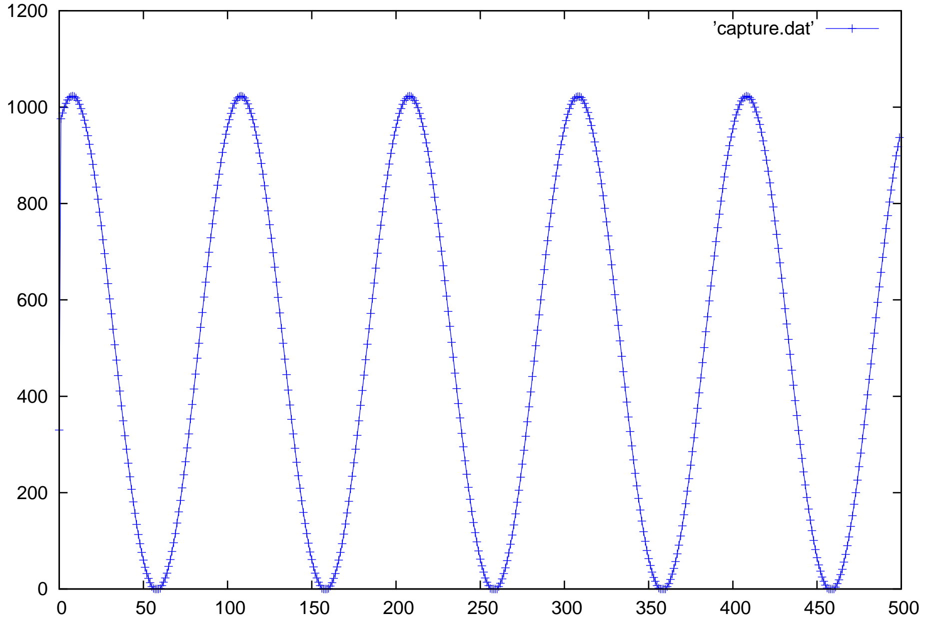
EBB Plot
