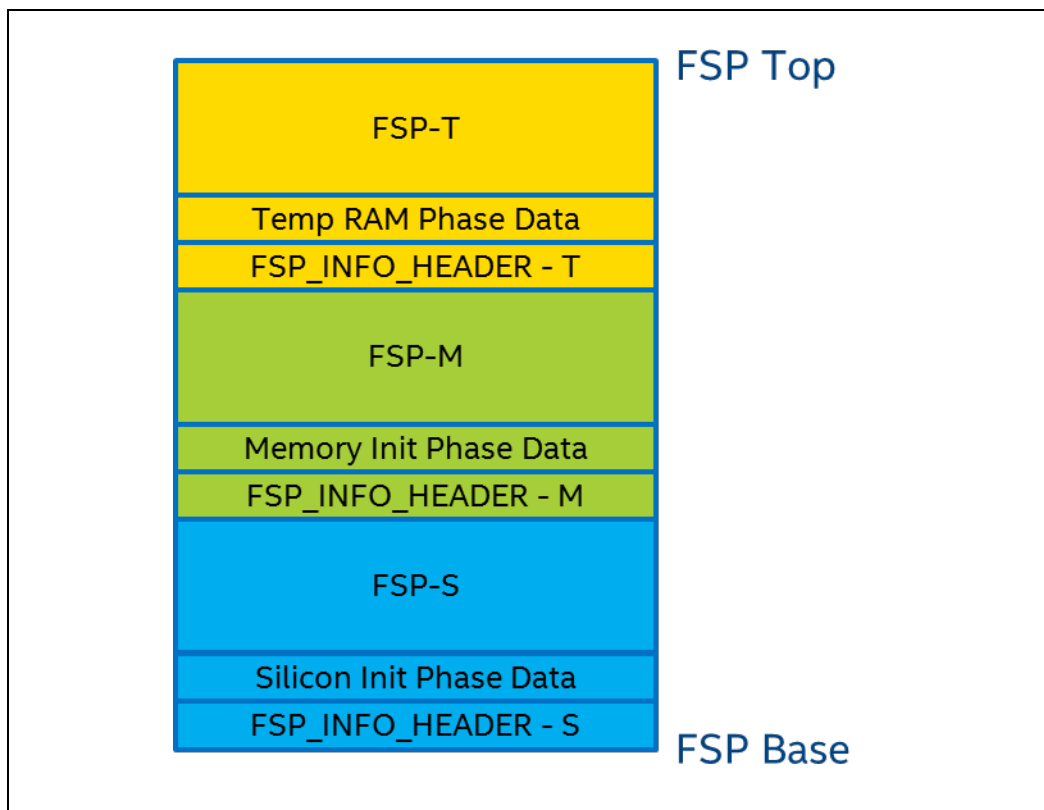
Figure 1. FSP Component Layout View
