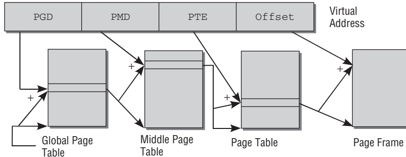
Figure 1-7: Splitting a virtual address.
