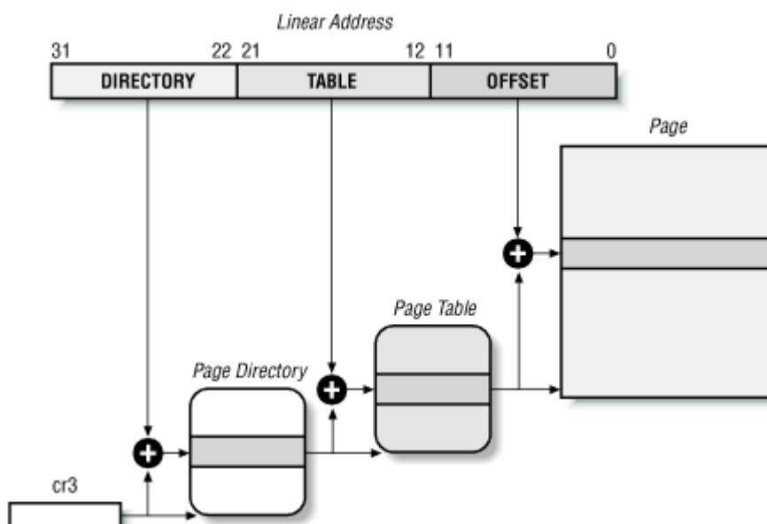
Figure 2-5. Paging by Intel 80x86 processors
