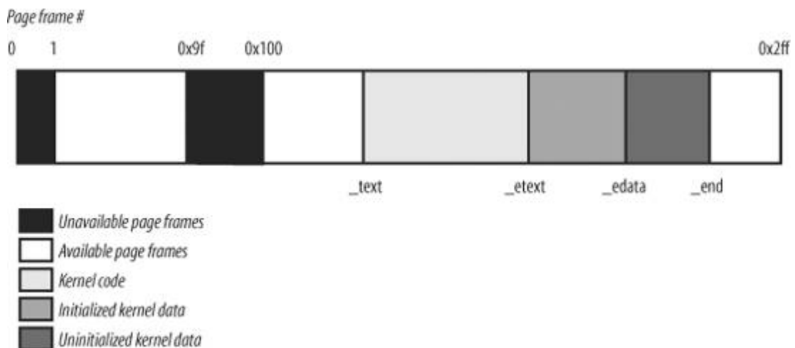
Figure 2-13. The first 768 page frames (3 MB) in Linux 2.6
