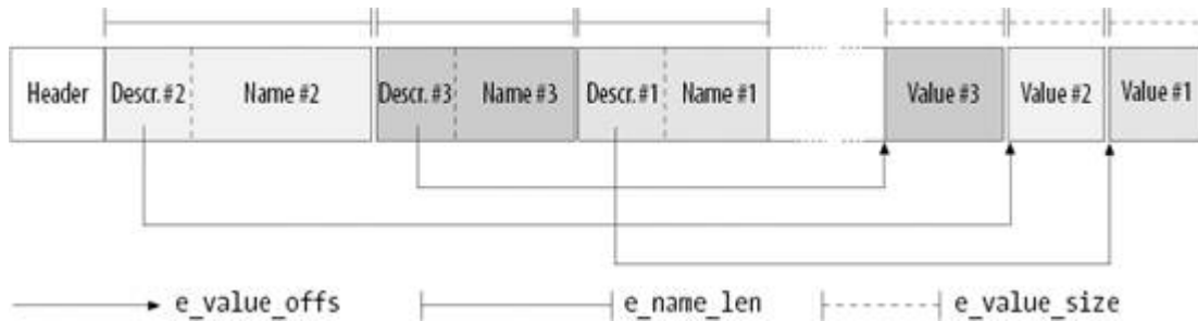
Figure 18-2. Layout of a block containing extended attributes
