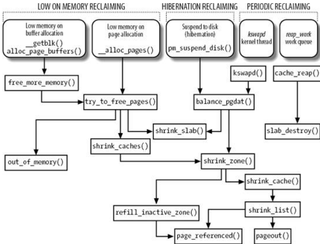
Figure 17-3. The main functions of the PFRA
