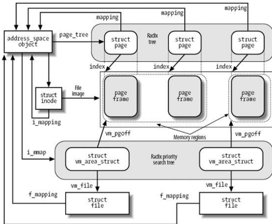
Figure 16-2. Data structures for file memory mapping
