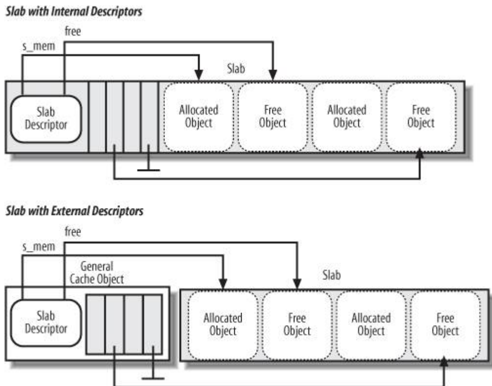
Figure 8-5. Relationships between slab and object descriptors
