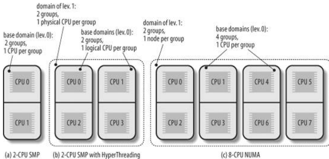
Figure 7-2. Three examples of scheduling domain hierarchies
