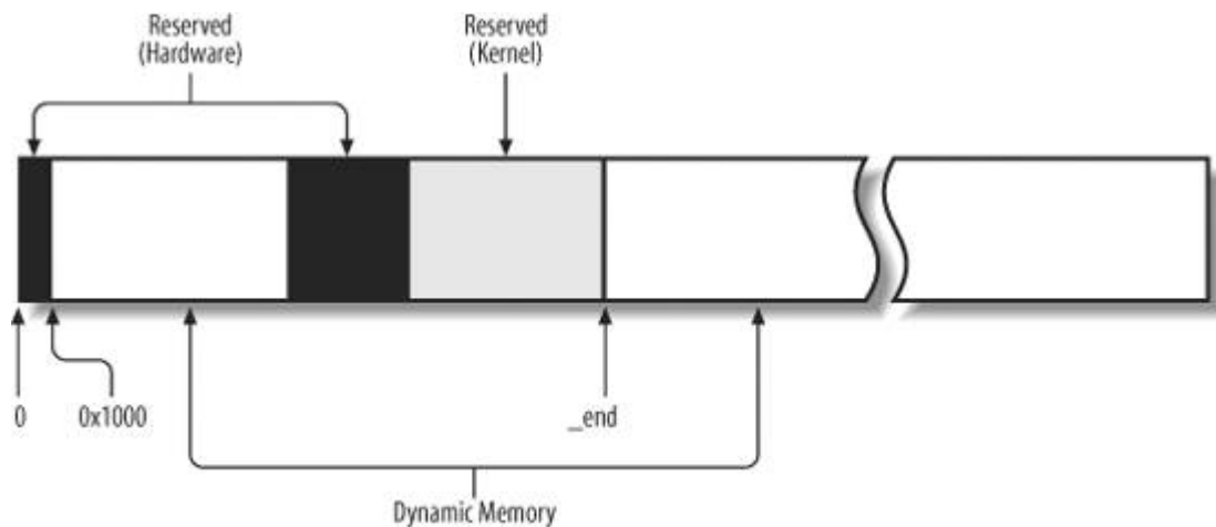
Figure 8-1. Dynamic memory
