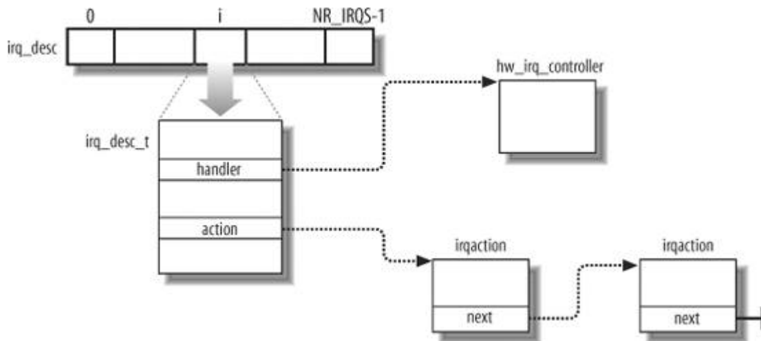
Figure 4-5. IRQ descriptors
