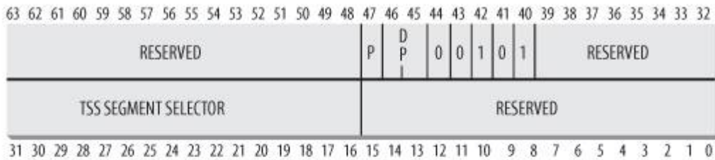
Figure 4-2. Gate descriptors' format
