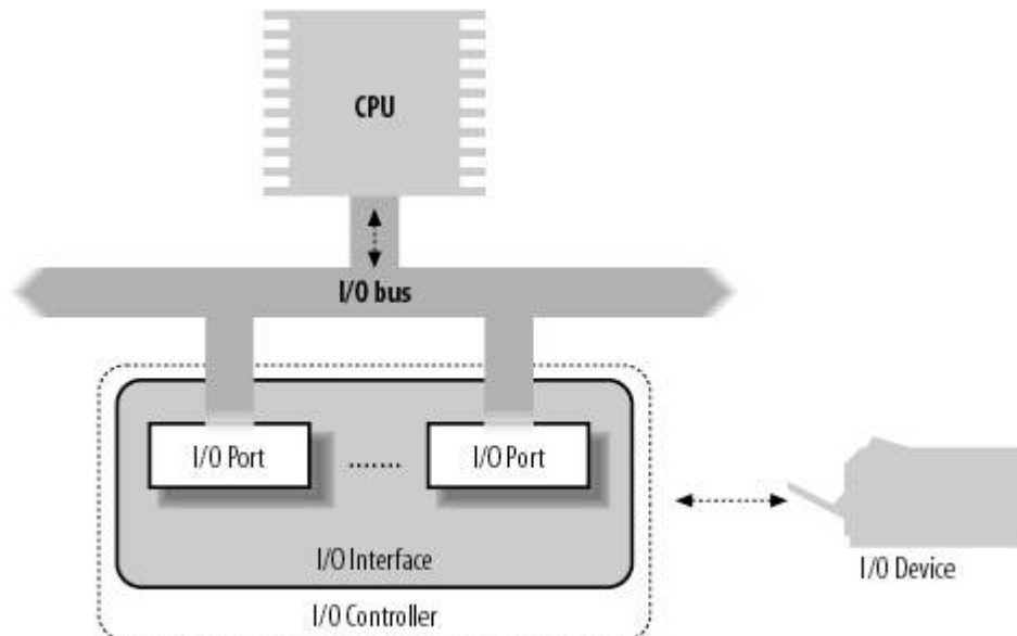
Figure 13-1. PC's I/O architecture
