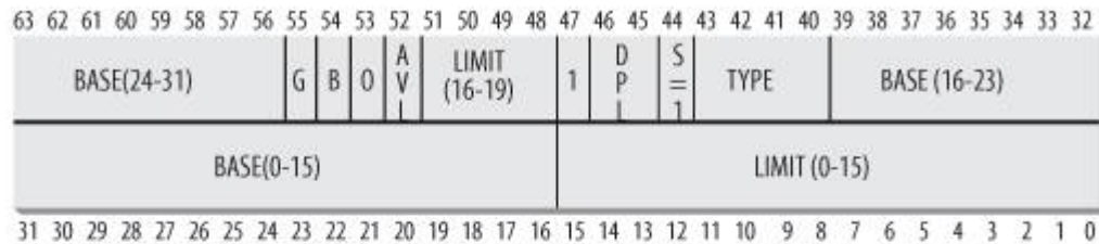
Figure 2-3. Segment Descriptor format
