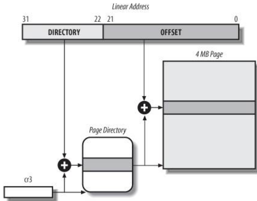
Figure 2-8. Extended paging
