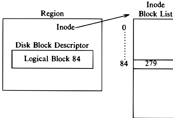
Figure 9.17. Mapping a File into a Region
