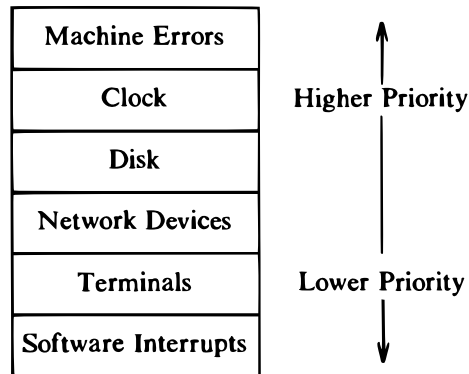
Figure 1.6. Typical Interrupt Levels
