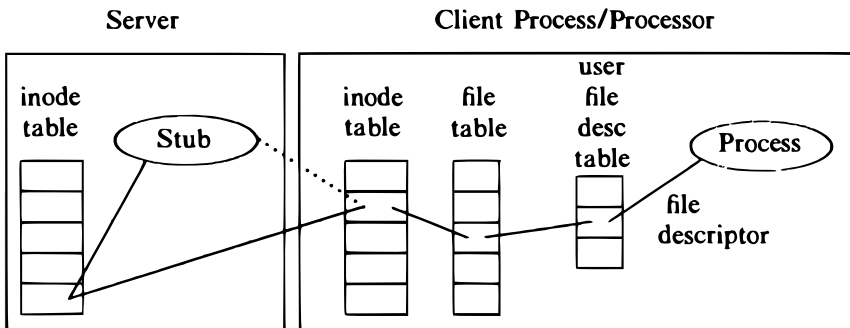
Figure 13.11. Opening a Remote File
