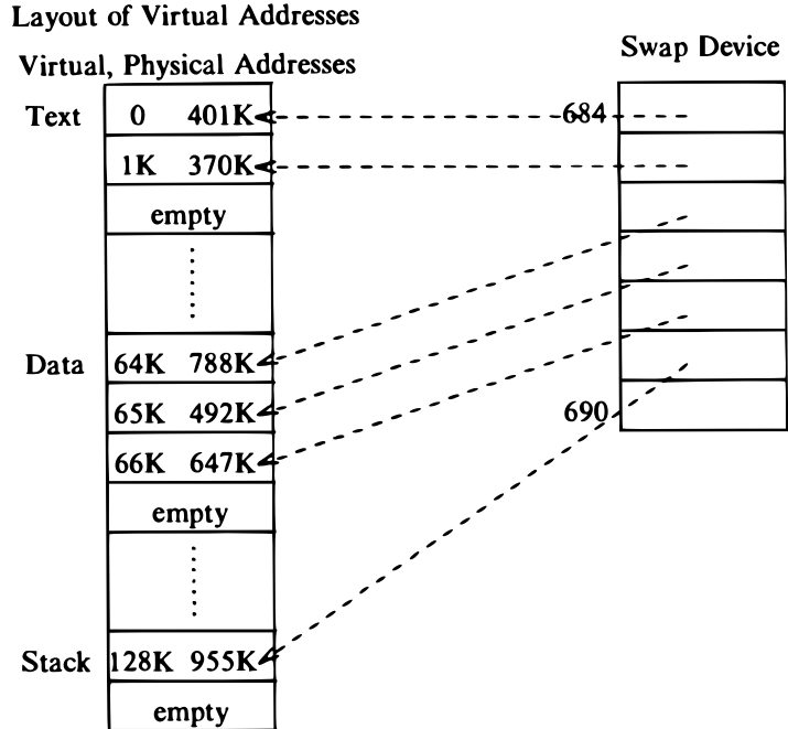
Figure 9.7. Swapping a Process into Memory
