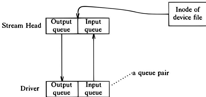
Figure 10.20. A Stream after Open
