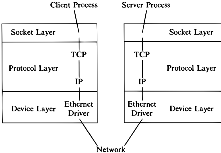
Figure 11.18. Sockets Model
