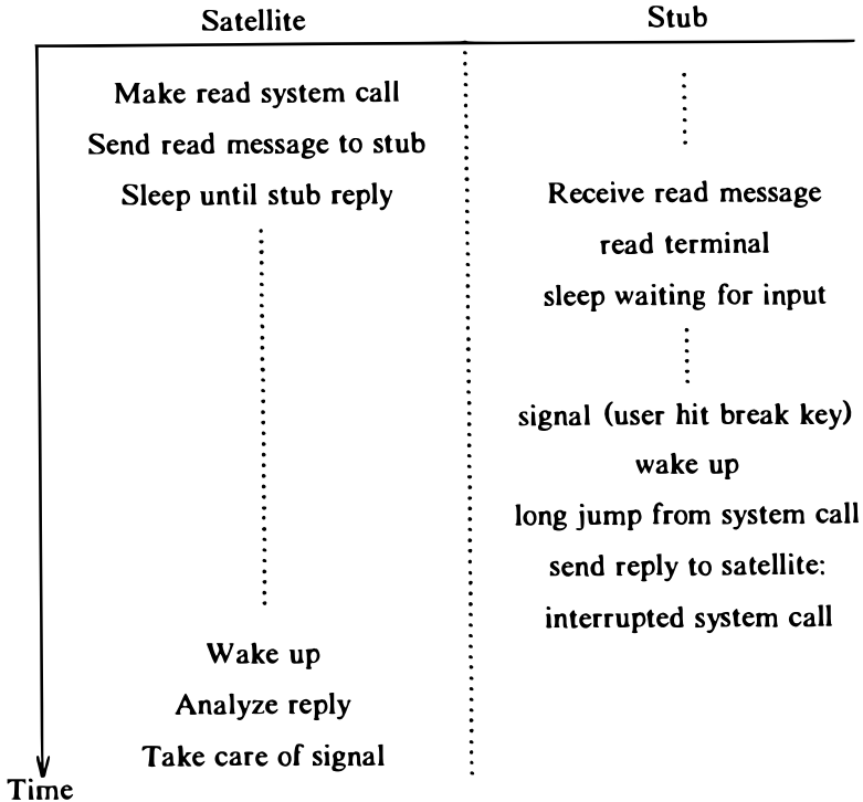
Figure 13.8. Interrupt in Middle of a System Call
