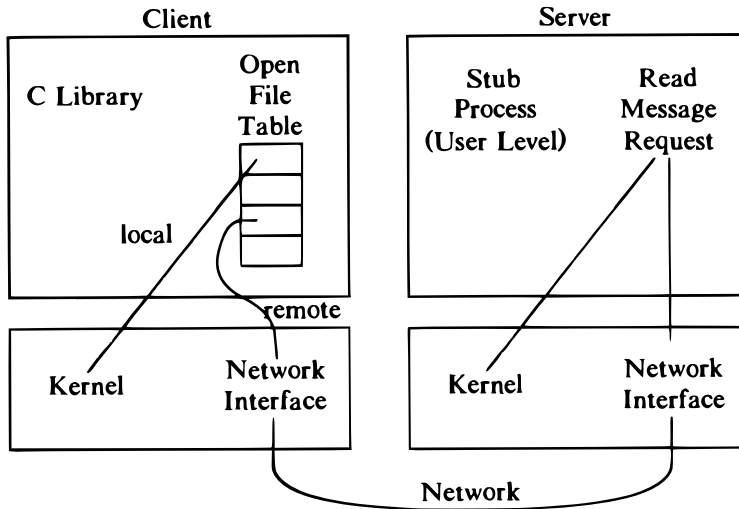
Figure 13.9. Formulation of File Service Requests
