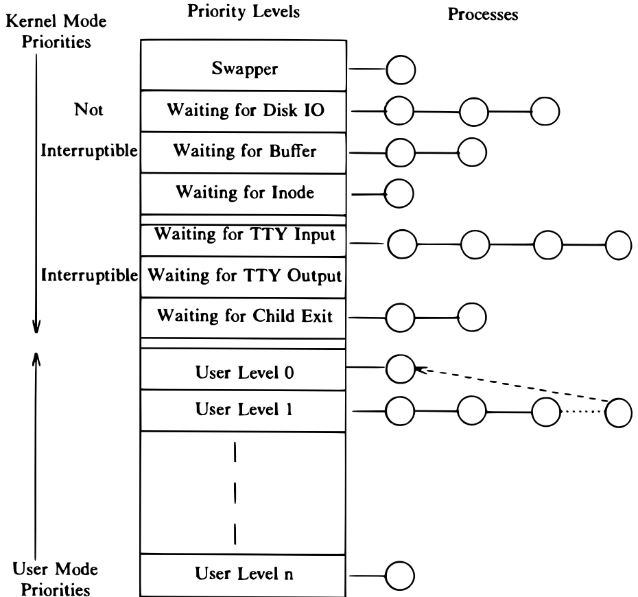
Figure 8.3. Movement of a Process on Priority Queues
