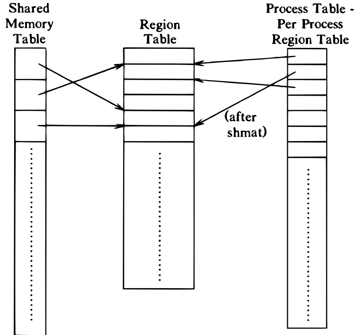
Figure 11.9. Data Structures for Shared Memory
