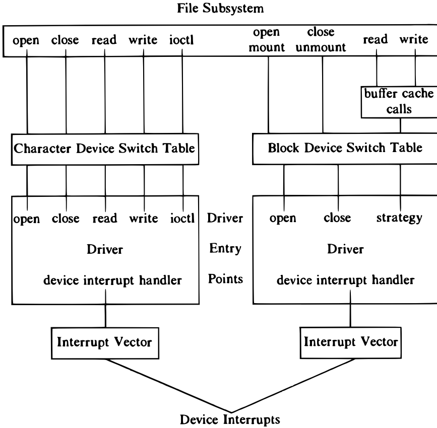
Figure 10.1. Driver Entry Points
