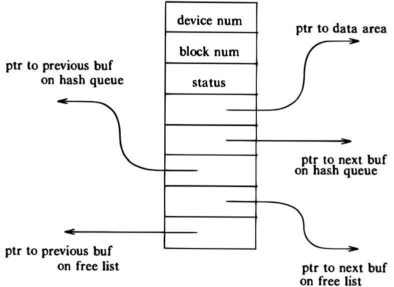
Figure 3.1. Buffer Header
