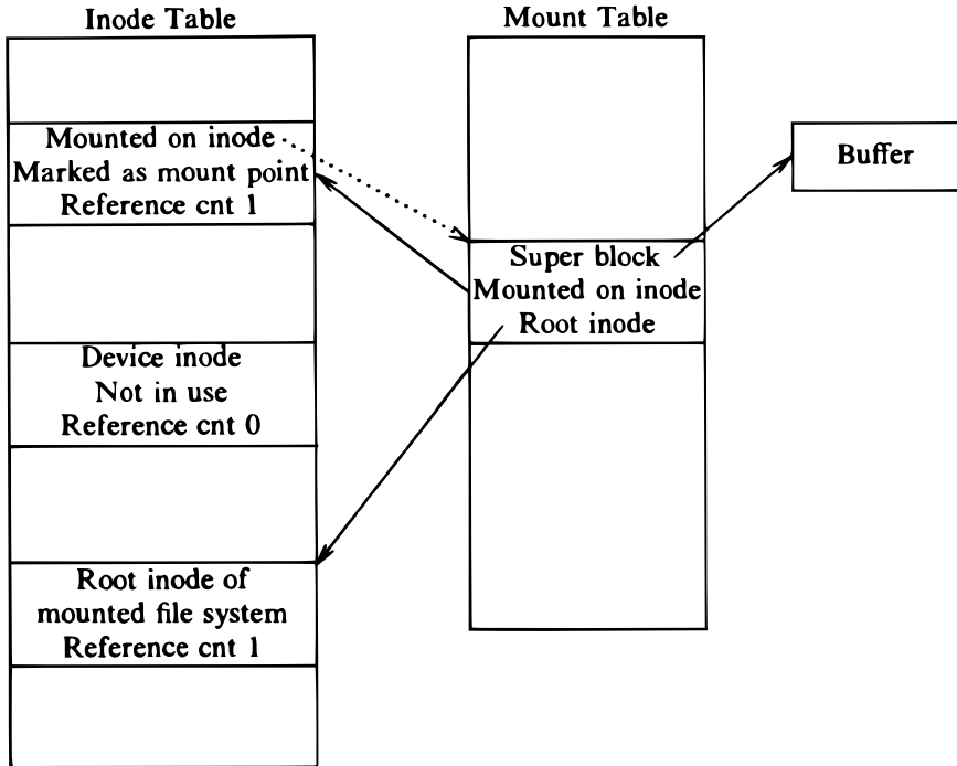
Figure 5.24. Data Structures after Mount
