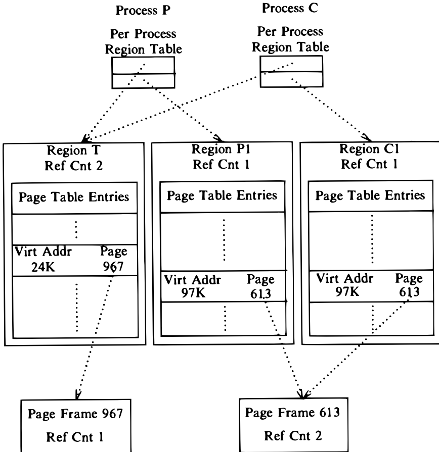
Figure 9.15. A Page in a Process that Forks
