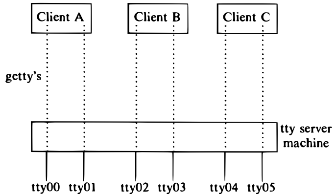
Figure 13.13. A Terminal Server Configuration
