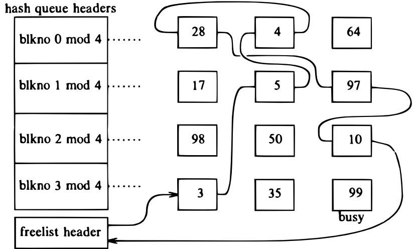
Search for Block 99, Block Busy
