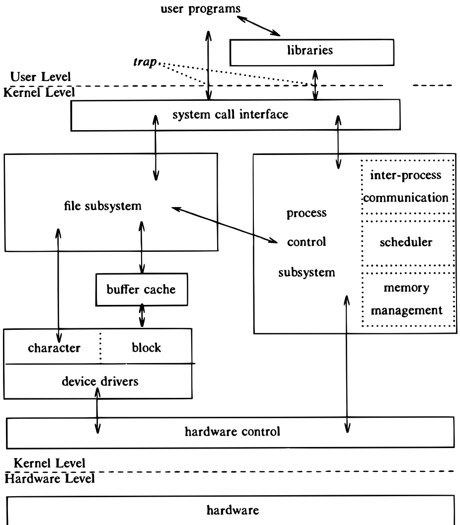
Figure 2.1. Block Diagram of the System Kernel
