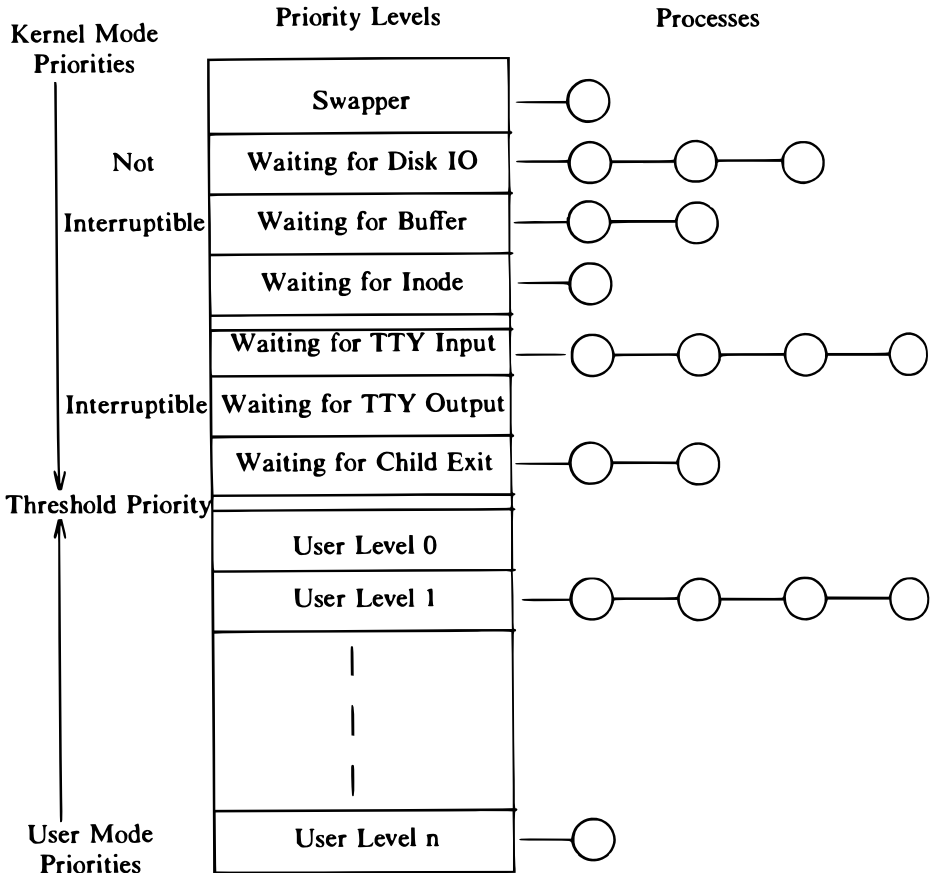
Figure 8.2. Range of Process Priorities
