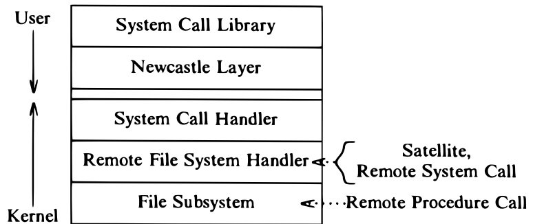
Figure 13.12. Conceptual Kernel Layer for Remote File Access
