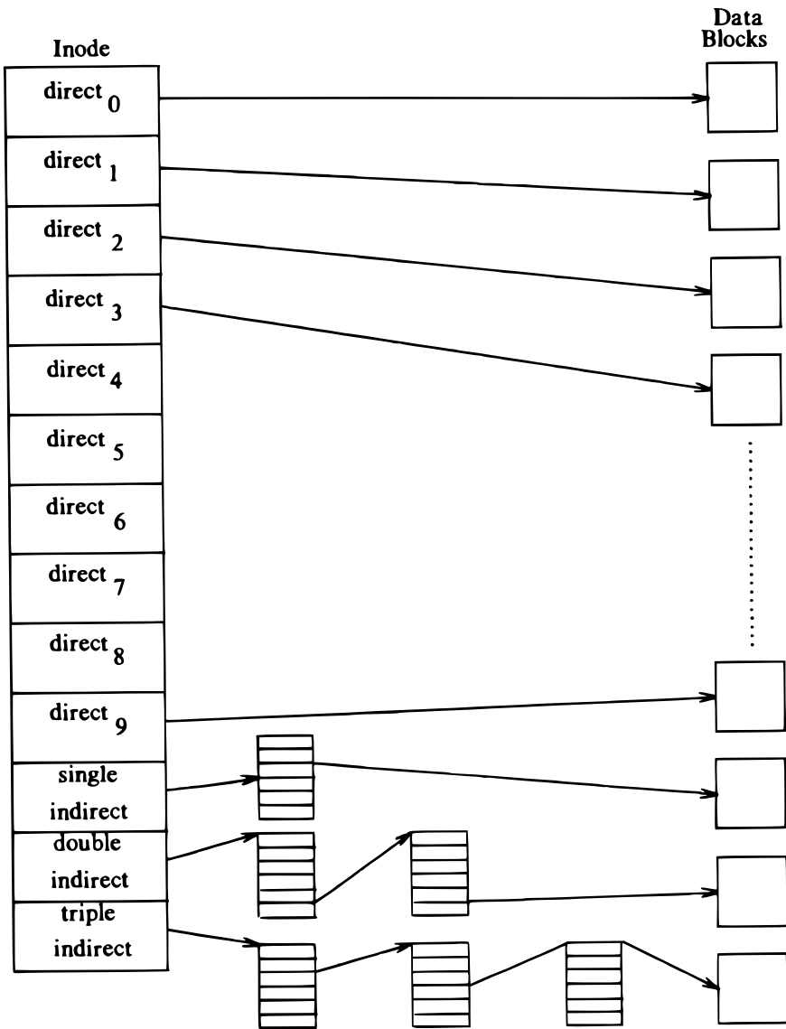
Figure 4.6. Direct and Indirect Blocks in Inode
