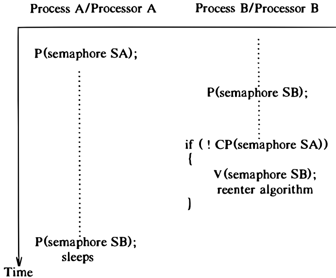
Figure 12.12. Use of Conditional P to Avoid Deadlock
