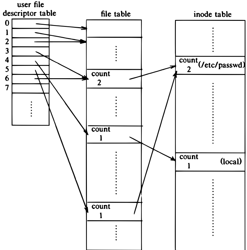
Figure 5.20. Data Structures after Dup
