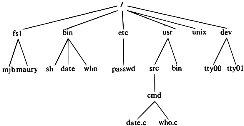
Figure 1.2. Sample File System Tree
