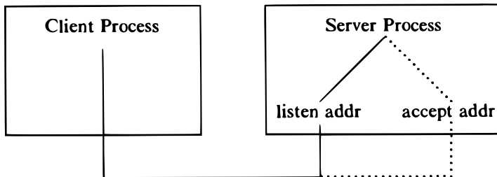
Figure 11.19. A Server Accepting a Call
