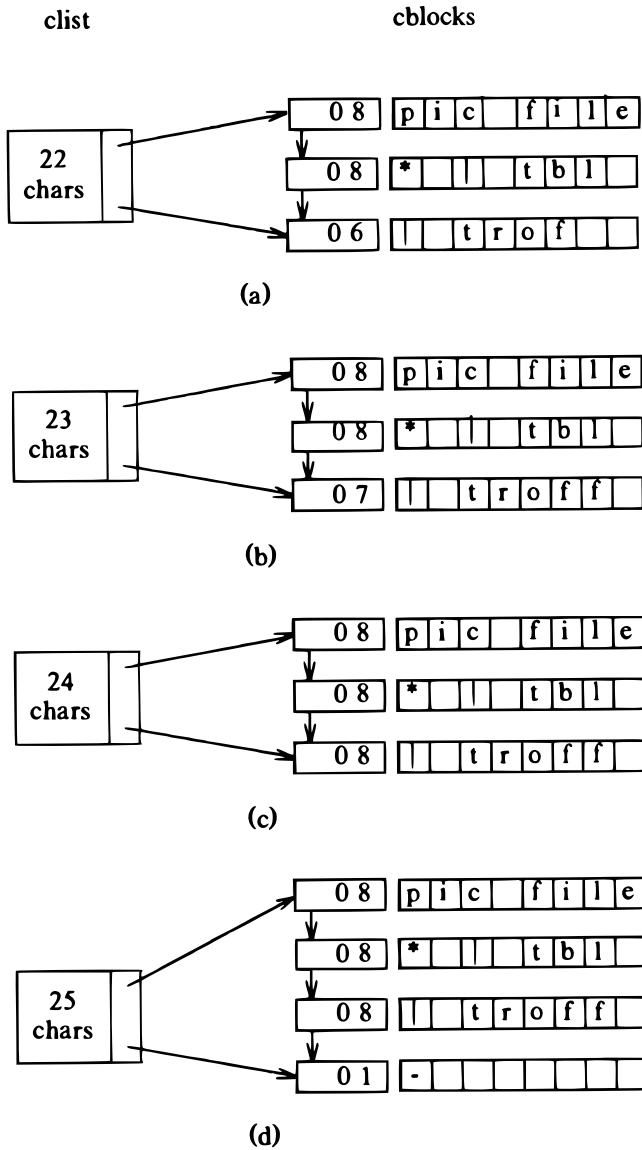
Figure 10.12. Placing a Character on a Clist
