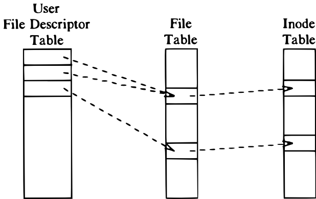
Figure 2.2. File Descriptors, File Table, and Inode Table
