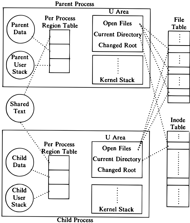
Figure 7.3. Fork Creating a New Process Context
