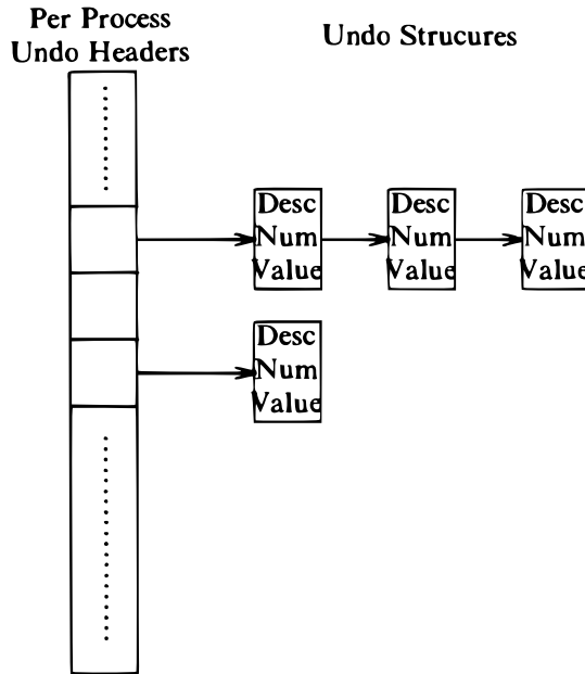
Figure 11.16. Undo Structures for Semaphores
