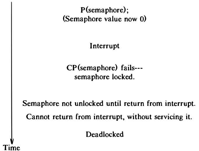
Figure 12.13. Deadlock in Interrupt Handler
