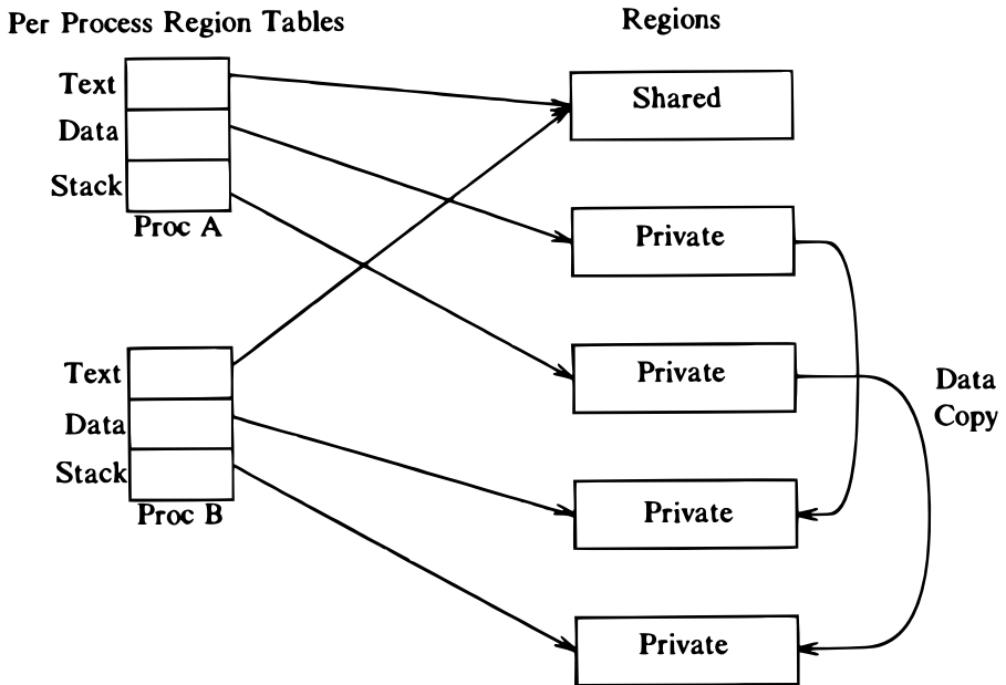
Figure 6.27. Duplicating a Region
