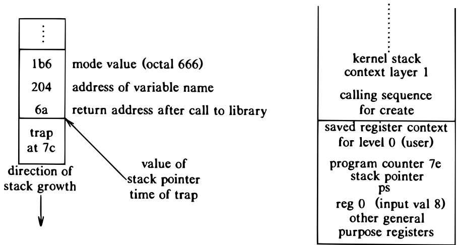
Figure 6.14. Stack Configuration for creat System Call
