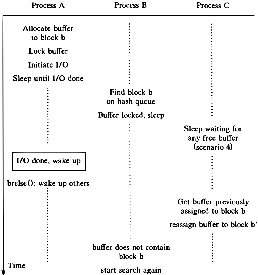
Figure 3.12. Race for a Locked Buffer
