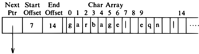
Figure 10.10. A Cblock
