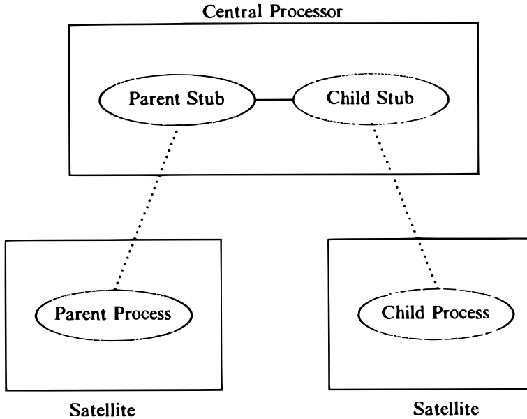
Figure 13.6. Fork on a Satellite Processor
