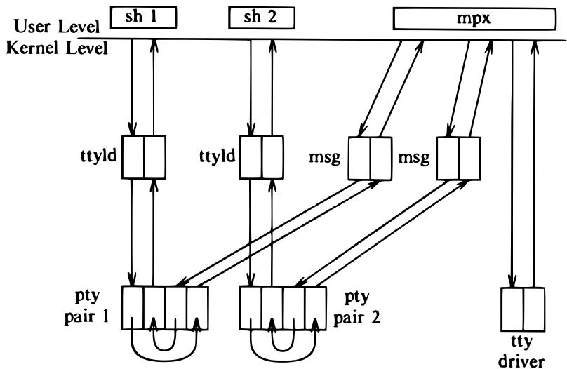
Figure 10.23. Windowing Virtual Terminals on a Physical Terminal
