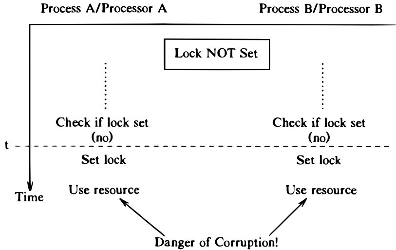
Figure 12.5. Race Conditions in Sleep-Locks on Multiprocessors
