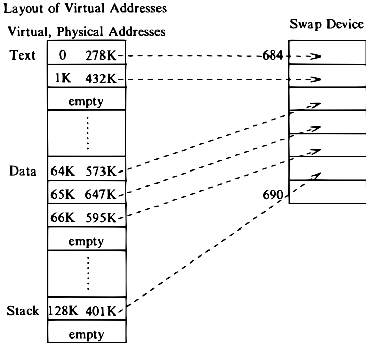
Figure 9.6. Mapping Process Space onto the Swap Device
