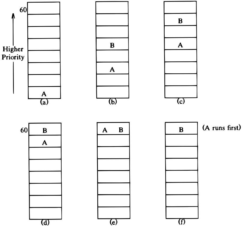
Figure 8.5. Round Robin Scheduling and Process Priorities
