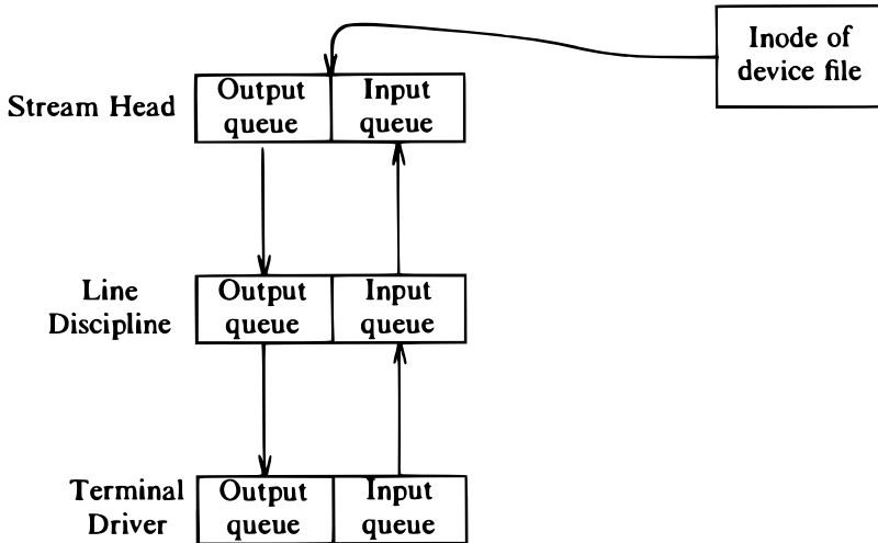
Figure 10.22. Pushing a Module onto a Stream
