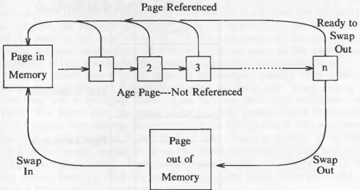
Figure 9.18. State Diagram for Page Aging
