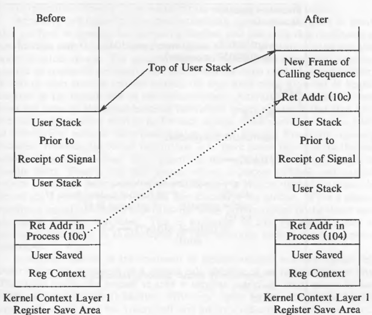
Figure 7.11. User Stack and Kernel Save Area Before and After Receipt of Signal
