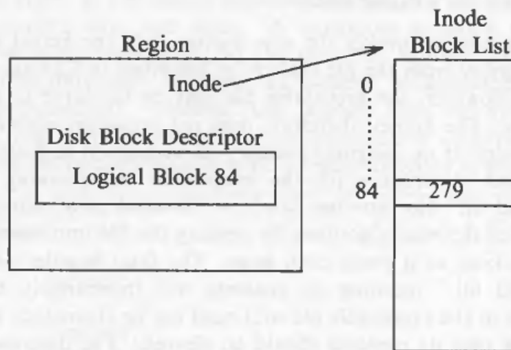
Figure 9.17. Mapping a File into a Region
