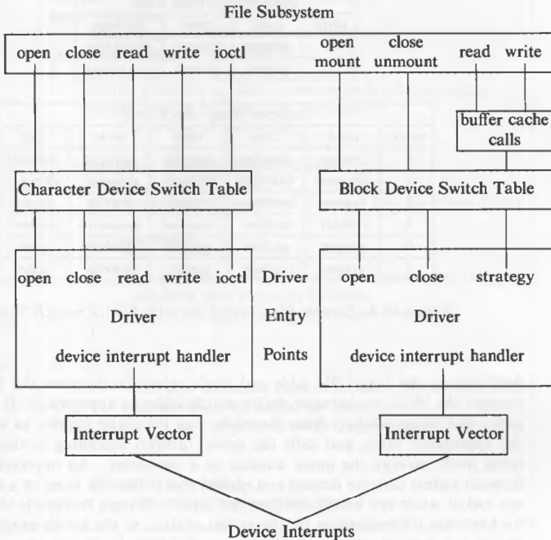
Figure 10.1. Driver Entry Points
