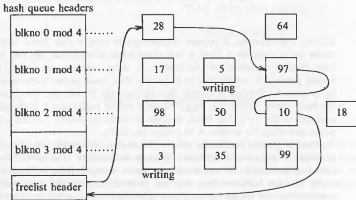
(b) Writing Blocks 3, 5, Reassign 4 to 18
