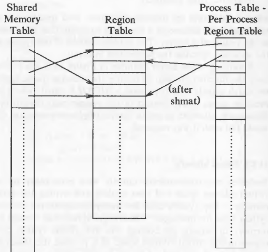
Figure 11.9. Data Structures for Shared Memory
