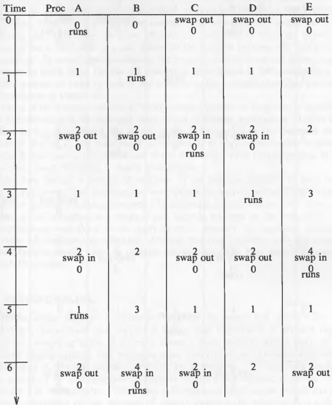
Figure 9.10. Sequence of Swapping Operations
