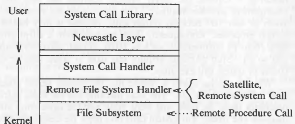
Figure 13.12. Conceptual Kernel Layer for Remote File Access
