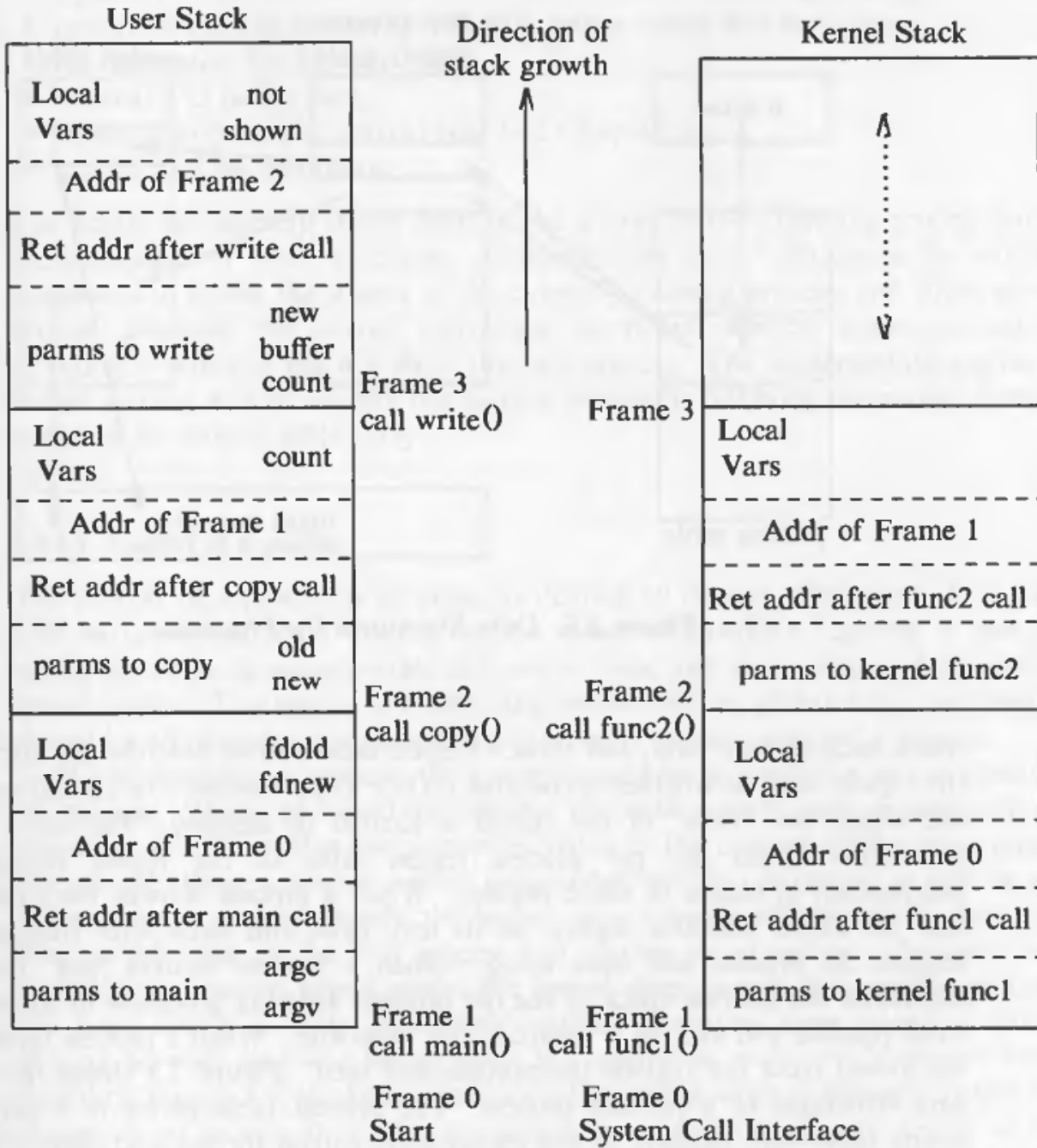
Figure 2.4. User and Kernel Stack for Copy Program
