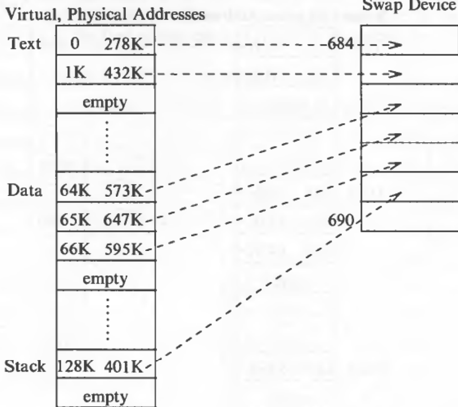
Figure 9.6. Mapping Process Space onto the Swap Device
