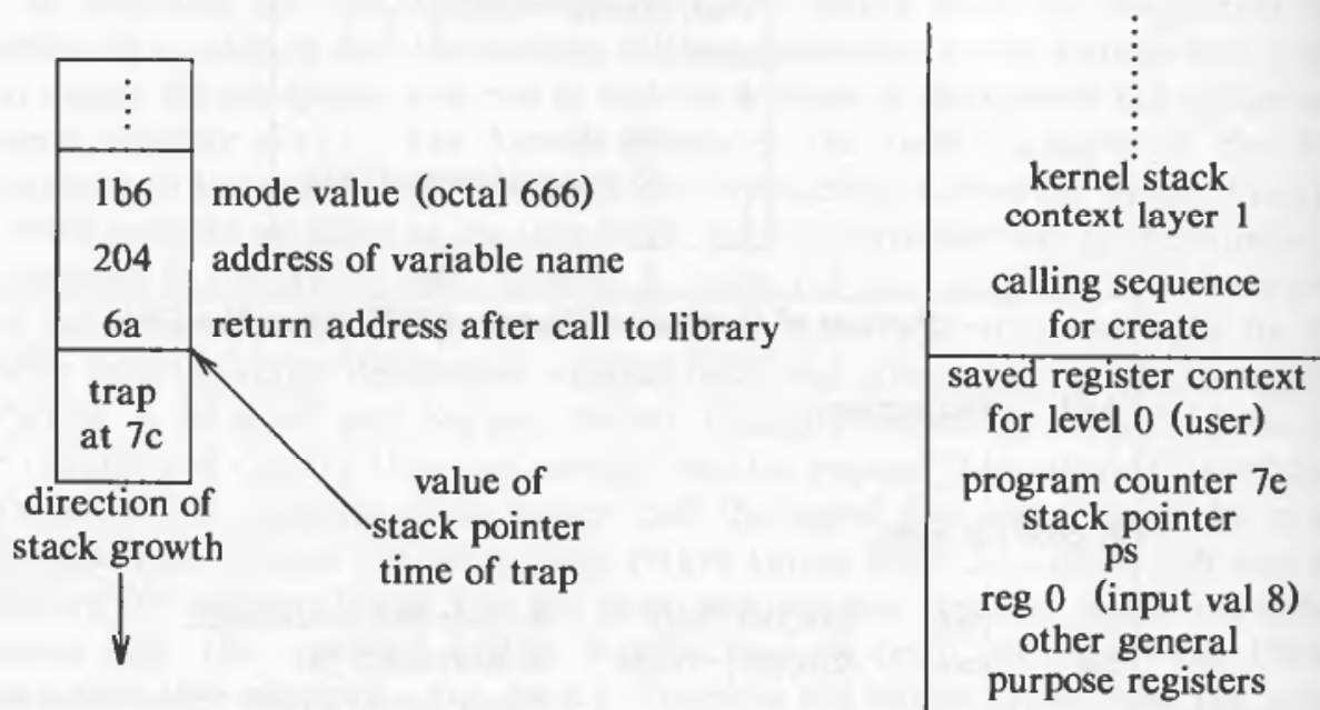
Figure 6.14. Stack Configuration for creat System Call
