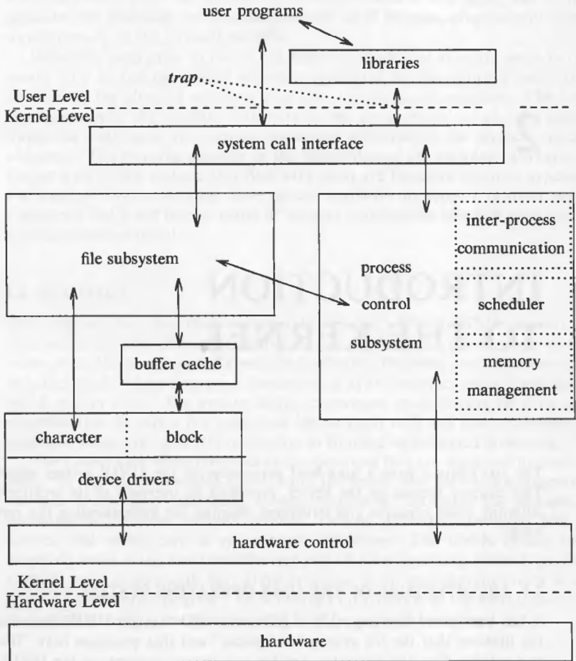
Figure 2.1. Block Diagram of the System Kernel
