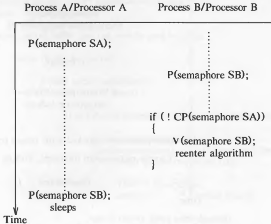
Figure 12.12. Use of Conditional P to Avoid Deadlock
