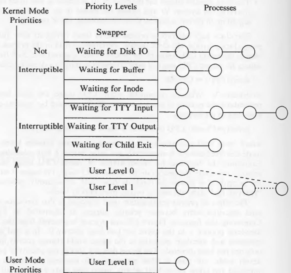
Figure 8.3. Movement of a Process on Priority Queues
