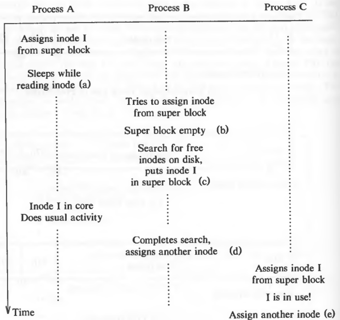
Figure 4.16. Race Condition in Assigning Inodes
