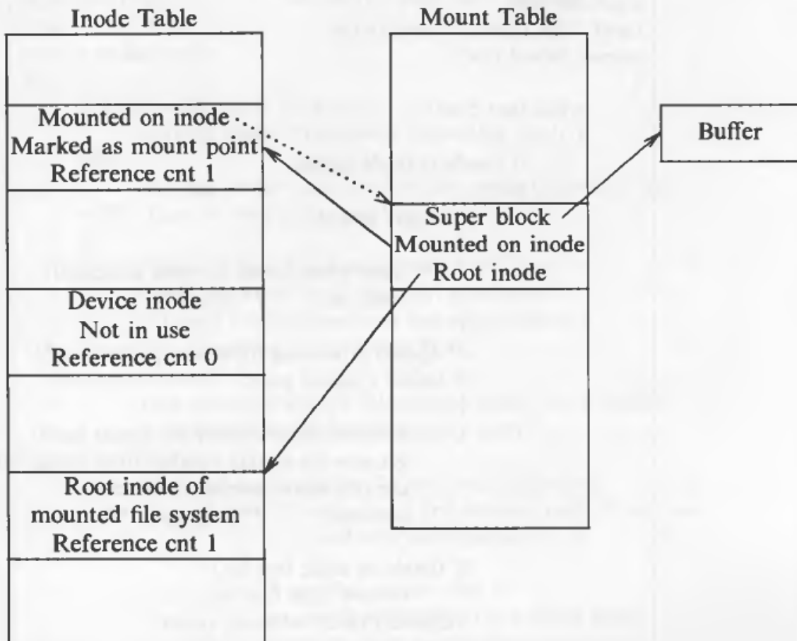
Figure 5.24. Data Structures after Mount
