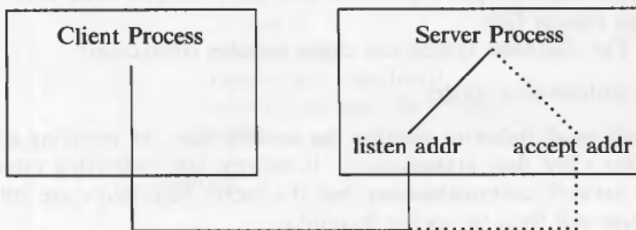
Figure 11.19. A Server Accepting a Call
