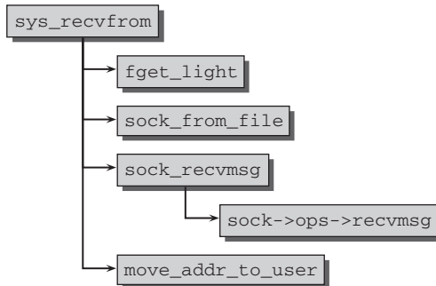
Figure 12-33: Code flow diagram for sys_recvfrom .
