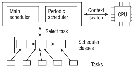
Figure 2-13: Overview of the components of the scheduling subsystem.
