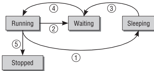
Figure 2-2: Transitions between process states.
