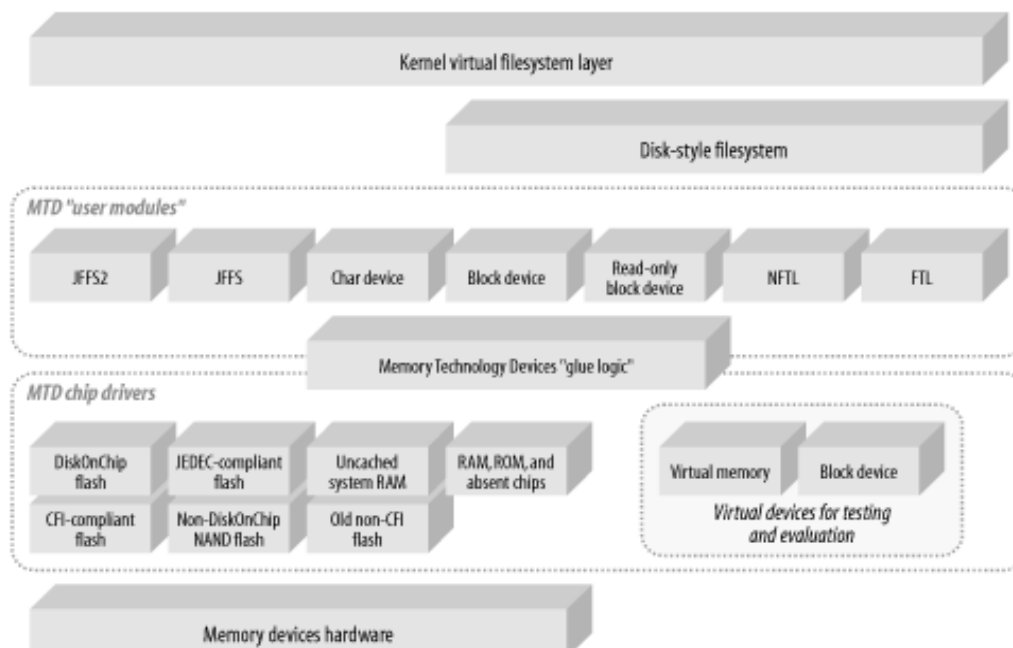
Figure 3-1. The MTD subsystem
