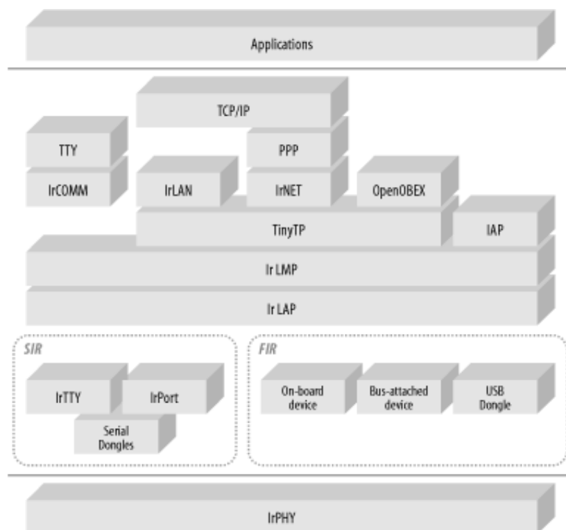
Figure 3-2. Linux IrDA subsystem architecture
