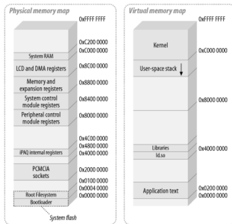
Figure 2-6. Physical and virtual memory maps for the Compaq iPAQ
