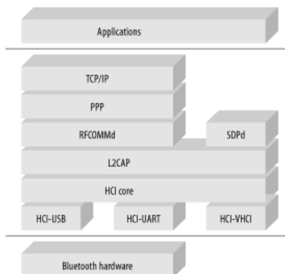
Figure 3-3. Linux BlueZ Bluetooth subsystem architecture
