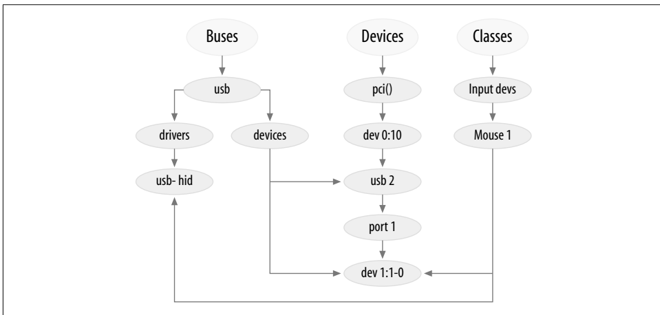
Figure 14-1. A small piece of the device model
