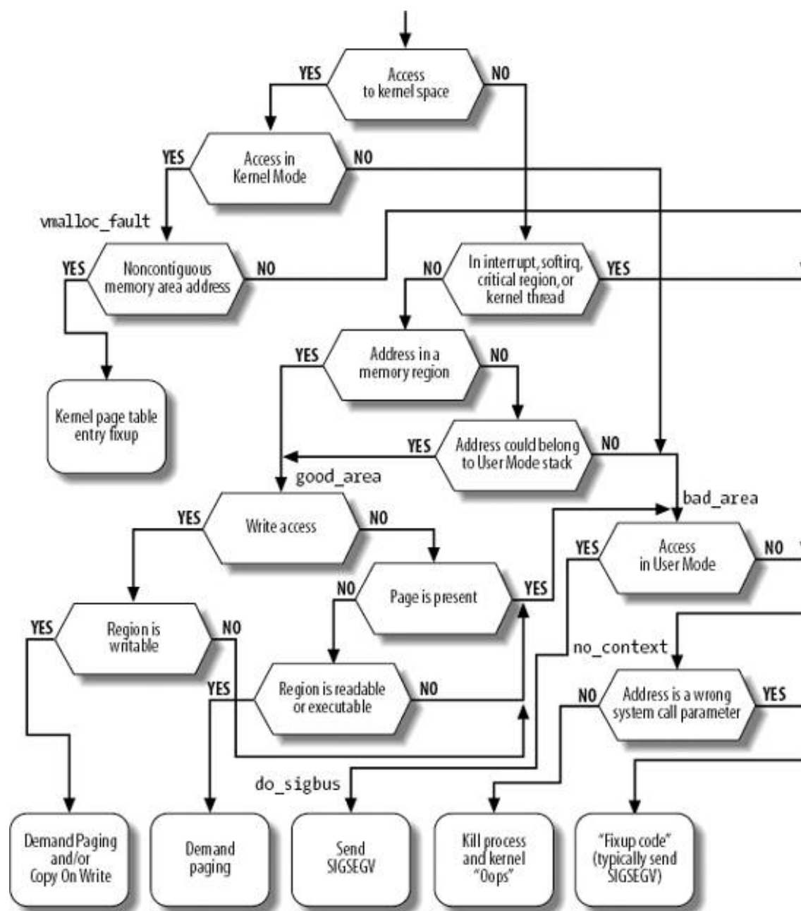
Figure 9-5. The flow diagram of the Page Fault handler
