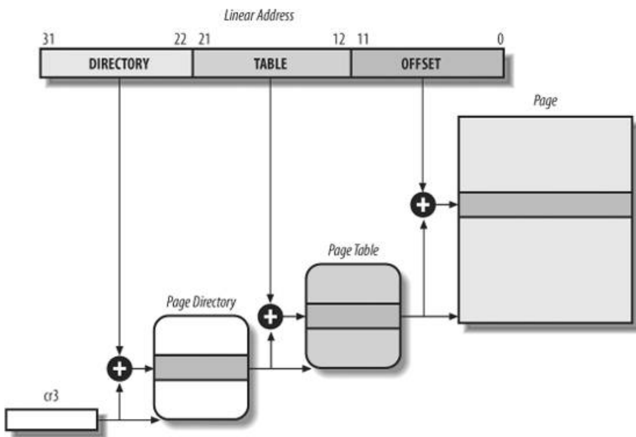
Figure 2-7. Paging by 80 x 86 processors
