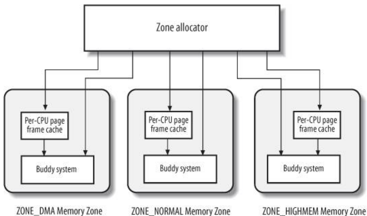
Figure 8-2. Components of the zoned page frame allocator
