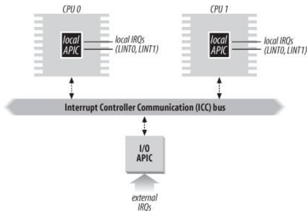
Figure 4-1. Multi-APIC system
