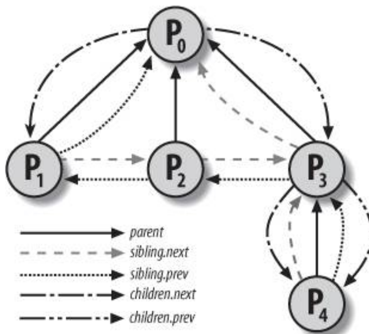
Figure 3-4. Parenthood relationships among five processes
