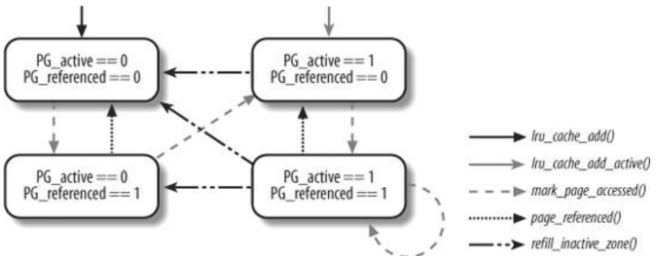
Figure 17-4. Moving pages across the LRU lists
