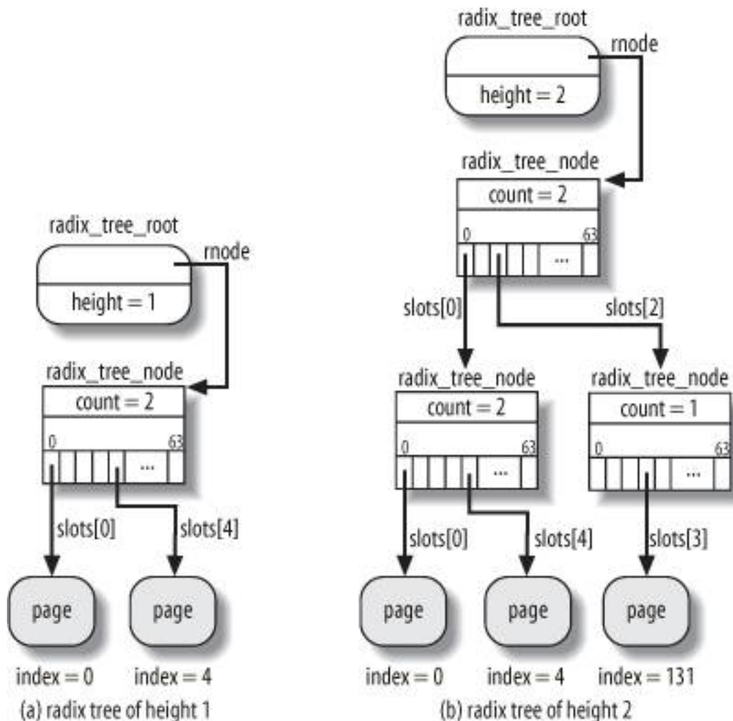
Figure 15-1. Two examples of a radix tree
