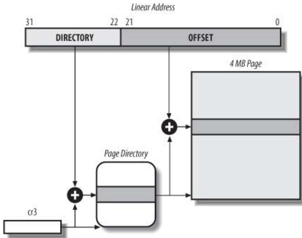
Figure 2-8. Extended paging
