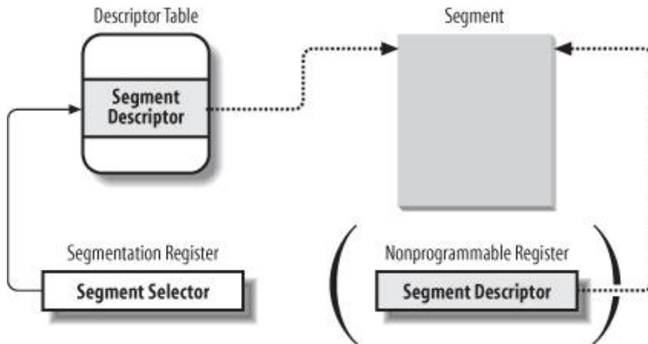
Figure 2-4. Segment Selector and Segment Descriptor
