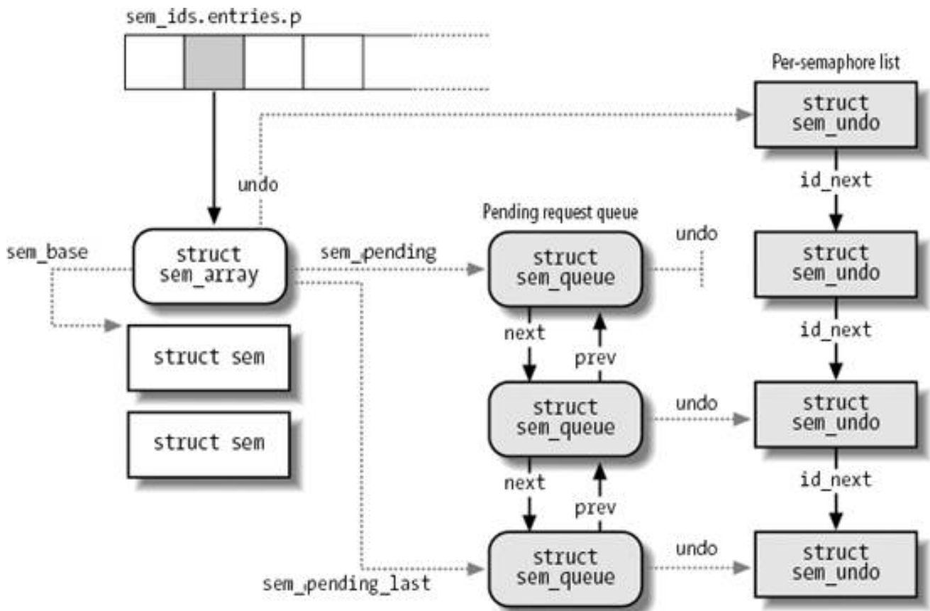
Figure 19-1. IPC semaphore data structures
