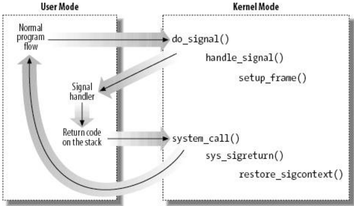
Figure 11-2. Catching a signal
