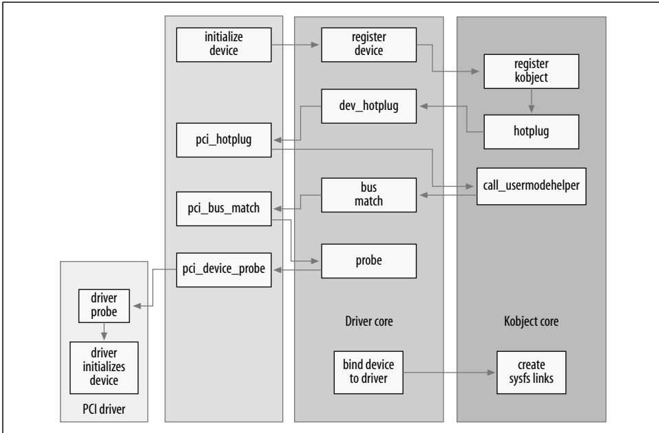
Figure 14-3. Device-creation process
