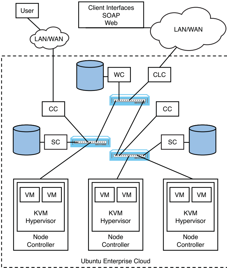
FIGURE 24.1 A sample UEC cloud.
