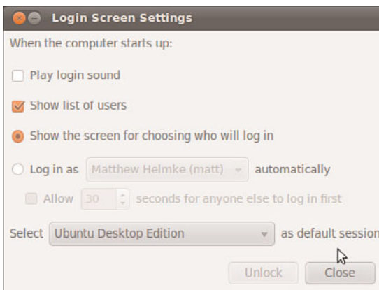
FIGURE 3.4 Configuring GDM.
