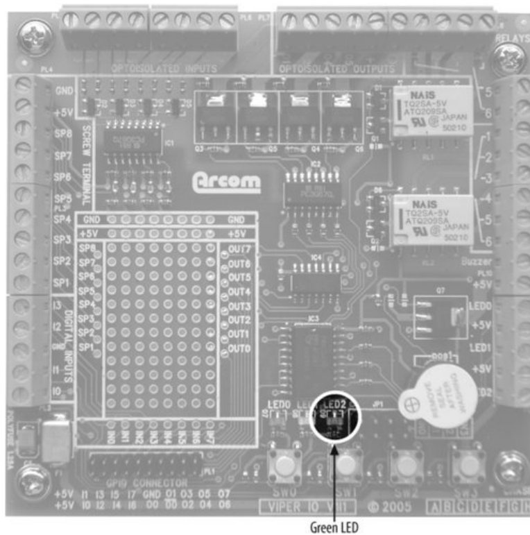
Figure 3-1. Arcrom board add-on module containing the green LED
