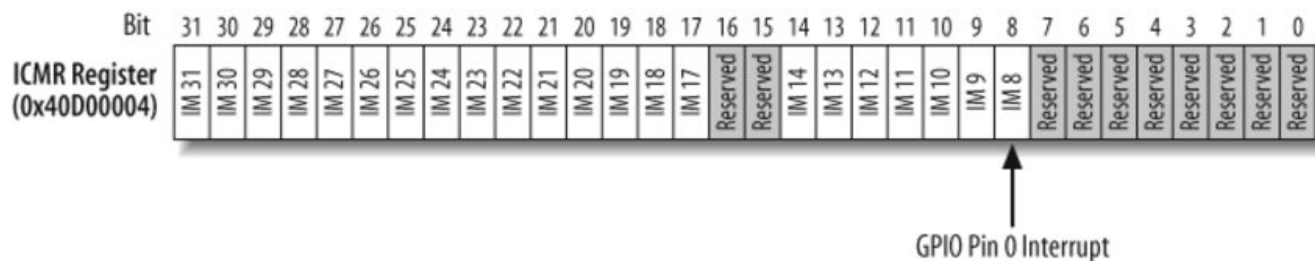
Figure 8-3. PXA255 Interrupt Controller Mask Register
