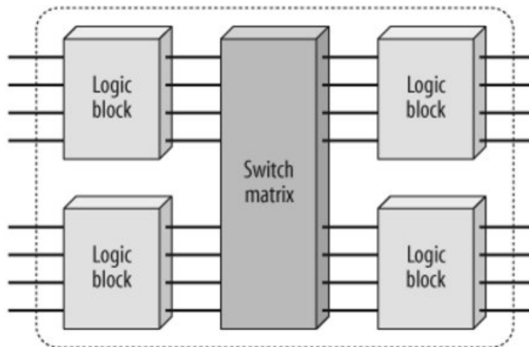
Figure 13-4. CPLD internal structure
