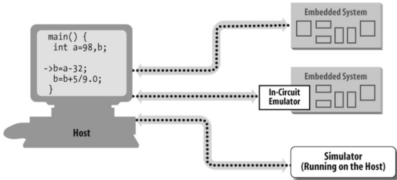
Figure 5-3. A common debugger frontend
