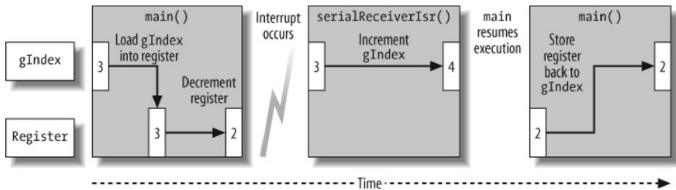
Figure 8-5. Example race condition
