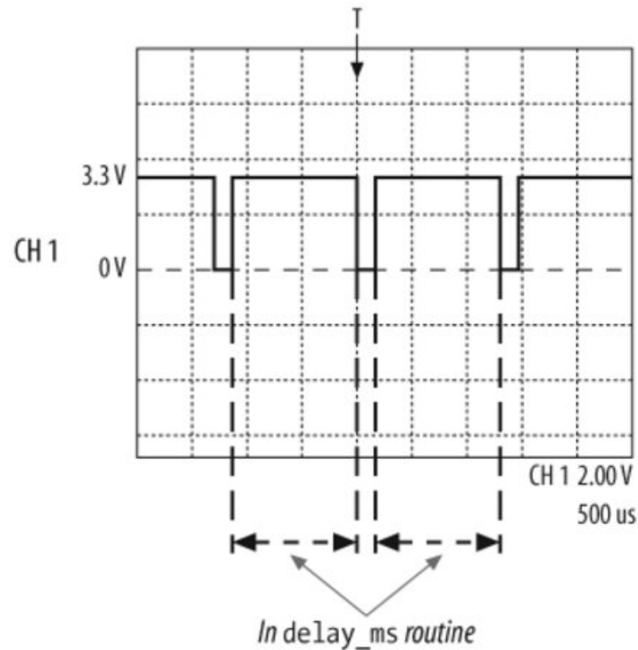
Figure 5-5. Using I/O signals for debug and performance measurements
