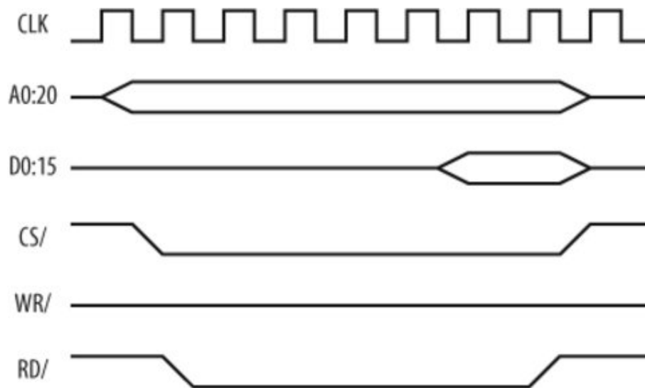
Figure 2-5. Example timing diagram
