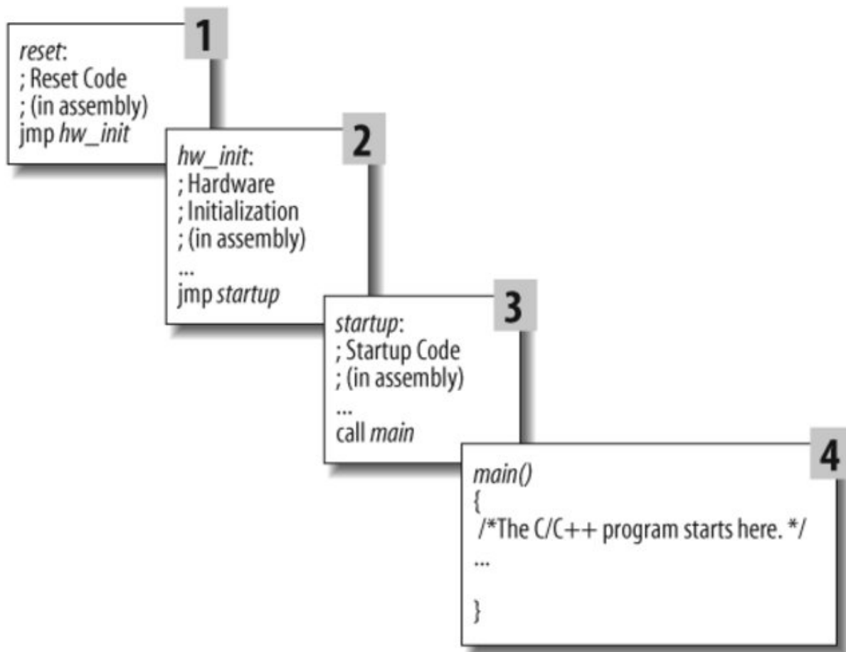
Figure 2-7. The hardware and software initialization process
