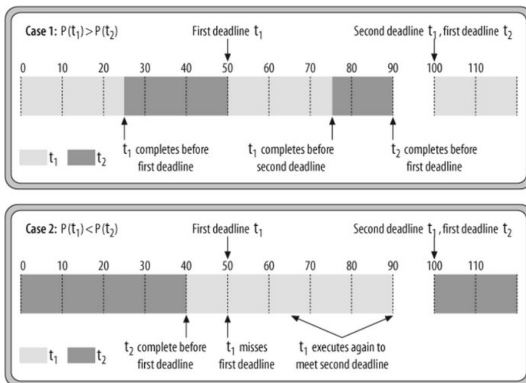
Figure 10-1. Scheduling outcome examples
