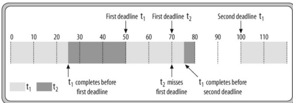
Figure 10-6. Example showing unschedulable task set
