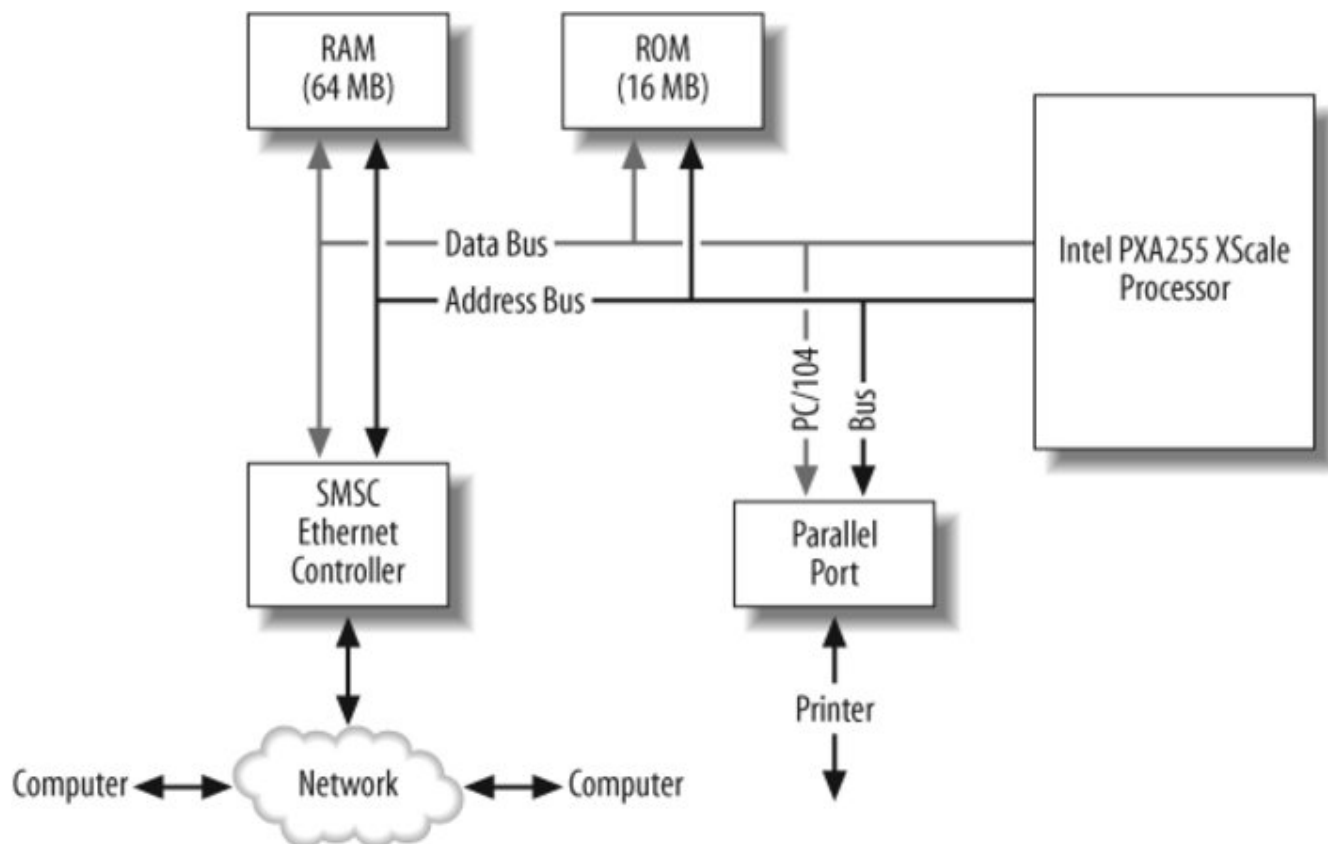
Figure 2-1. Block diagram for the print server
