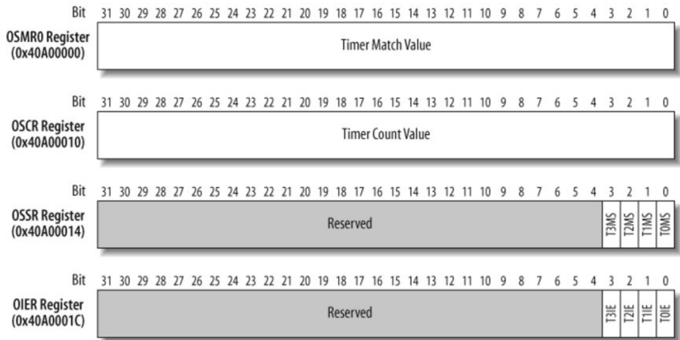
Figure 8-6. PXA255 processor timer 0 registers
