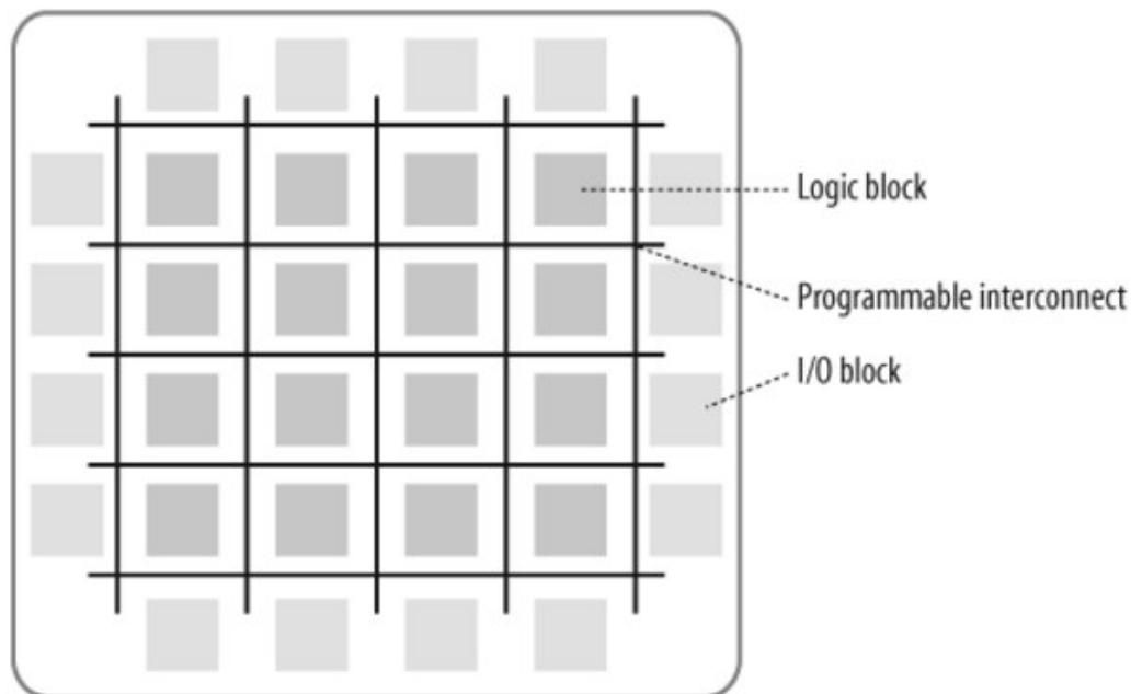
Figure 13-5. FPGA internal structure
