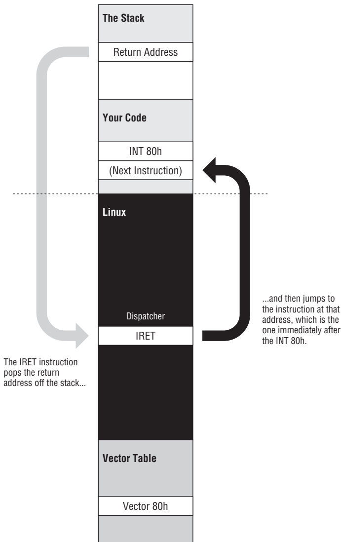
Figure 8-6: Returning home from an interrupt
