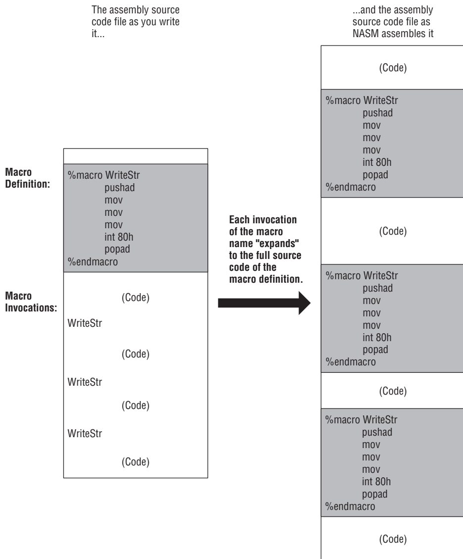
Figure 10-4: How macros work
