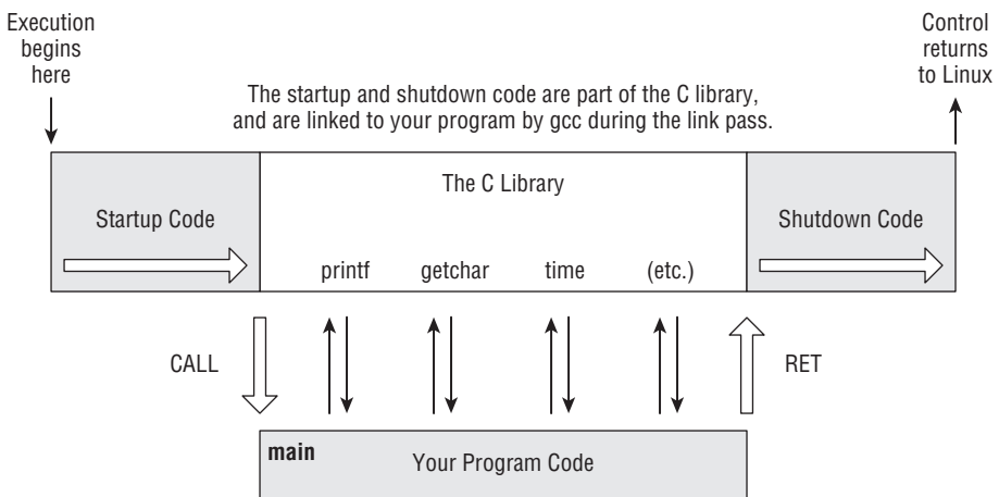
Figure 12-2: Structure of a hybrid C-assembly program
