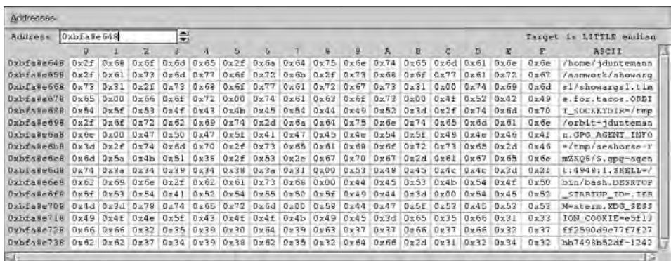
Figure 11-6: Command-line arguments in Insight’s Memory view
