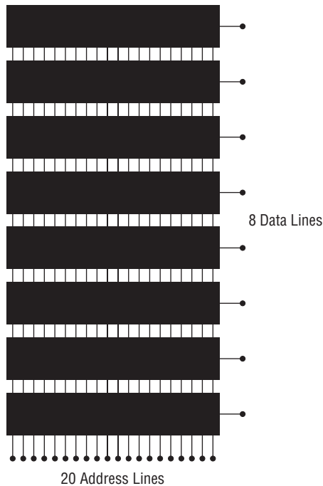
Figure 3-3: A 1-megabyte memory system
