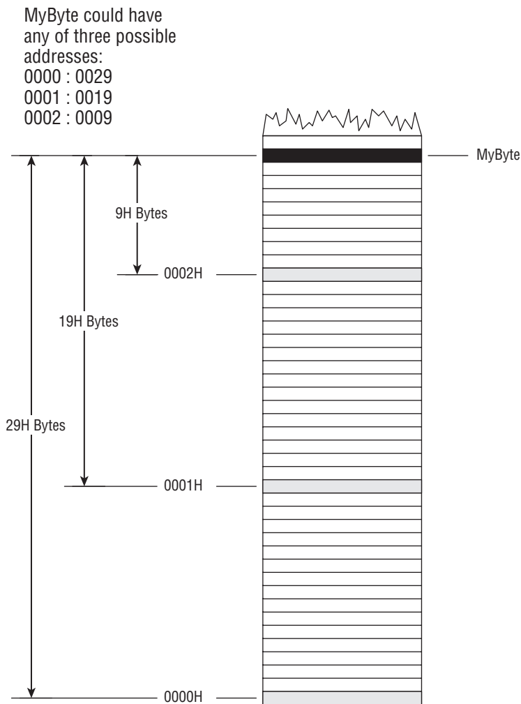
Figure 4-5: Segments and offsets
