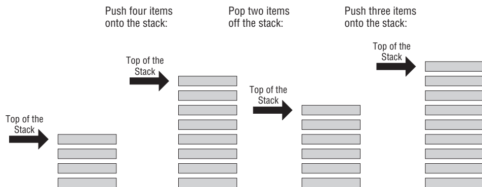
Figure 8-1: The stack
