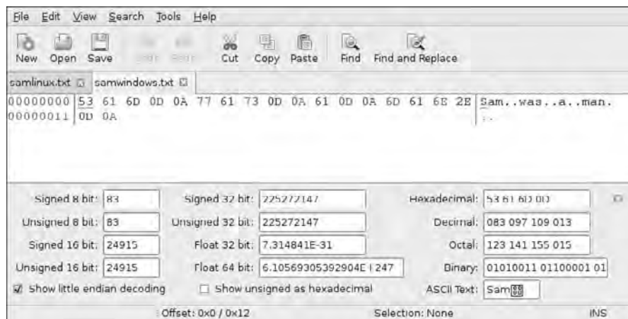
Figure 5-2: Displaying a Windows text file with the Bless editor
