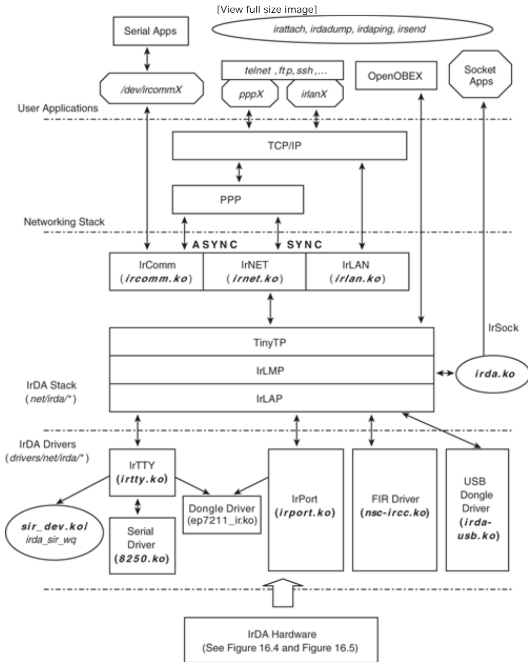
Figure 16.6. Communicating over Linux-IrDA.
