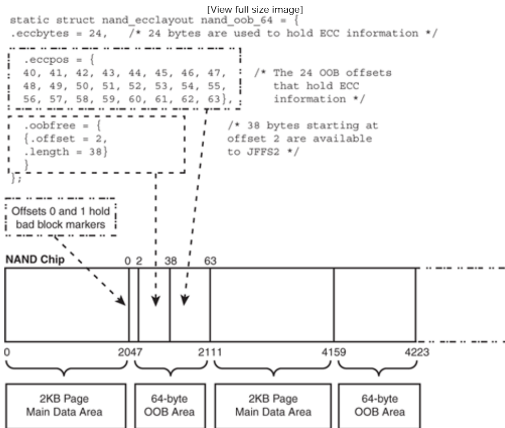
Figure 17.4. Layout of a NAND flash chip.
