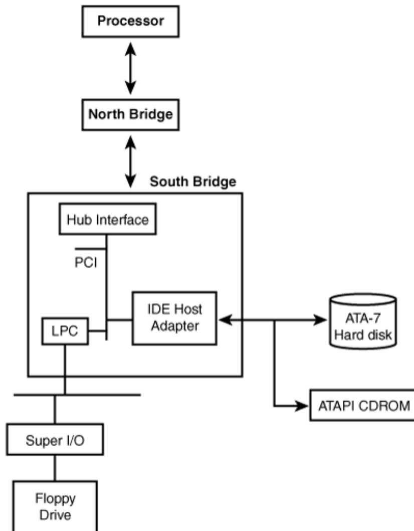
Figure 14.1. Storage media in a PC system.
