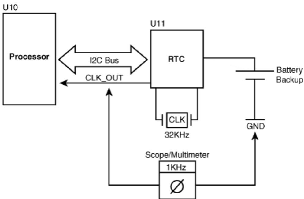
Figure 18.4. Debugging an I 2 C RTC on an embedded system.
