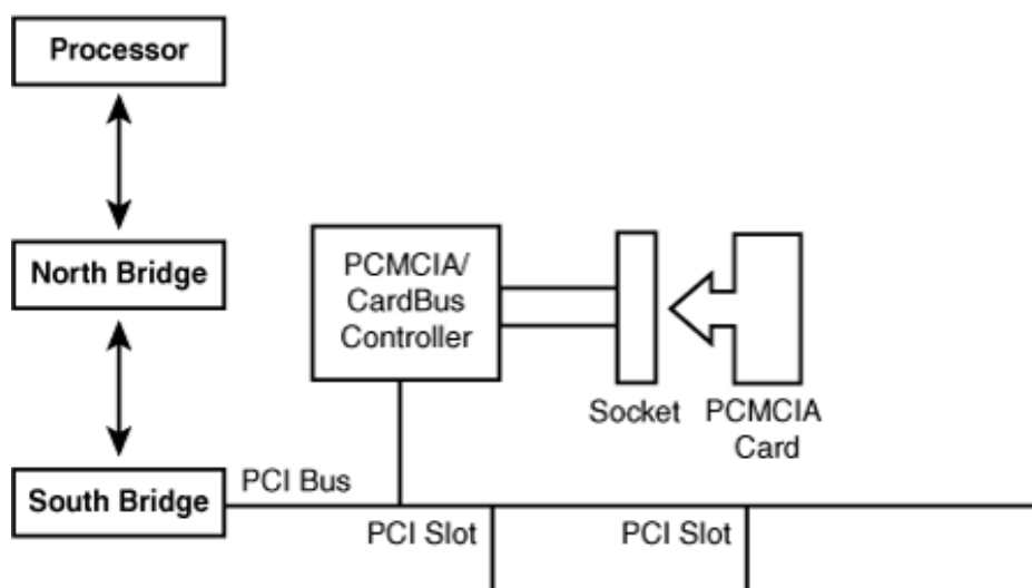
Figure 9.1. PCMCIA on a laptop.
