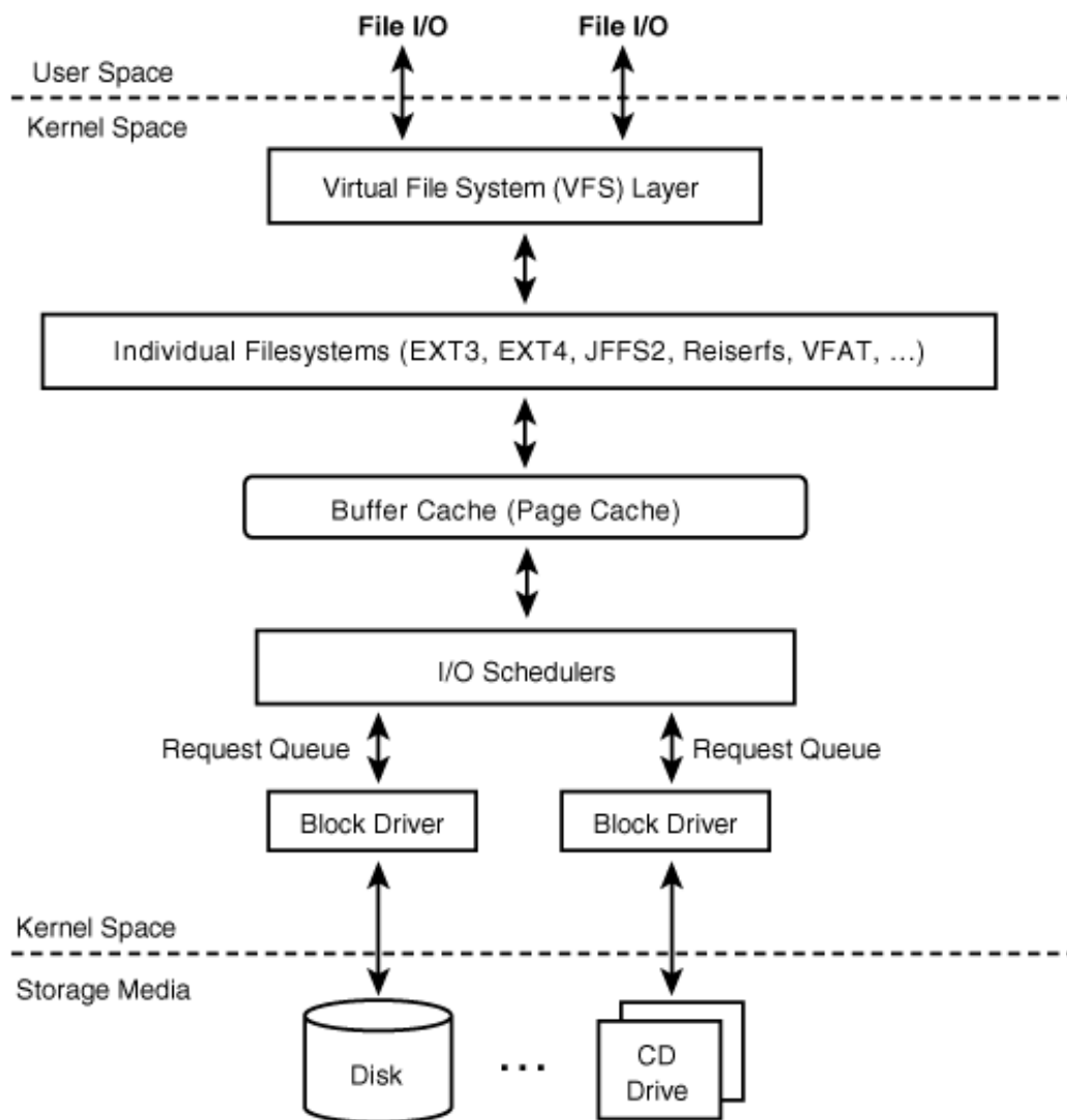
Figure 14.2. Block I/O on Linux.
