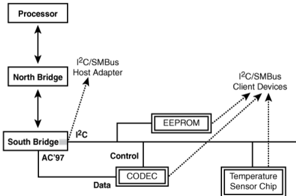
Figure 8.1. I 2 C/SMBus on PC-compatible hardware.
