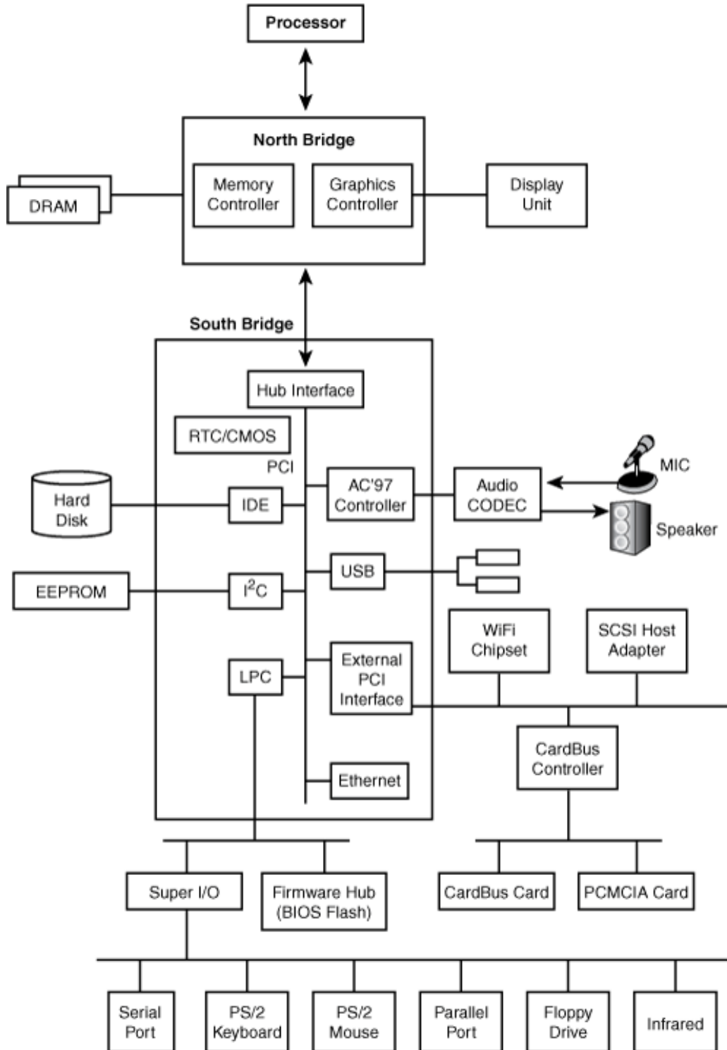
Figure 4.1. Hardware block diagram of a PC-compatible system.
