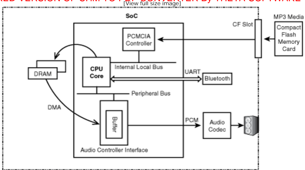
Figure 13.4. Audio on a Linux MP3 player.
