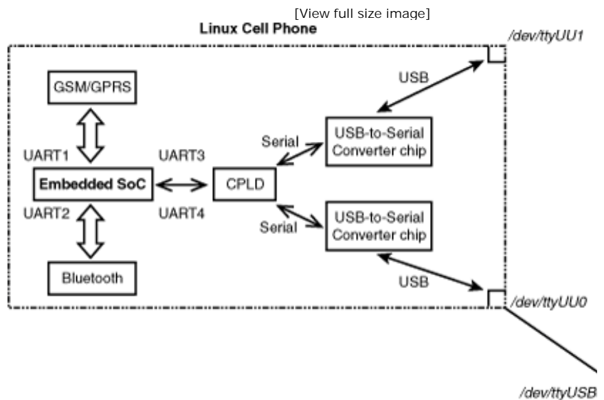
Figure 6.5. USB_UART ports on a Linux cell phone.
