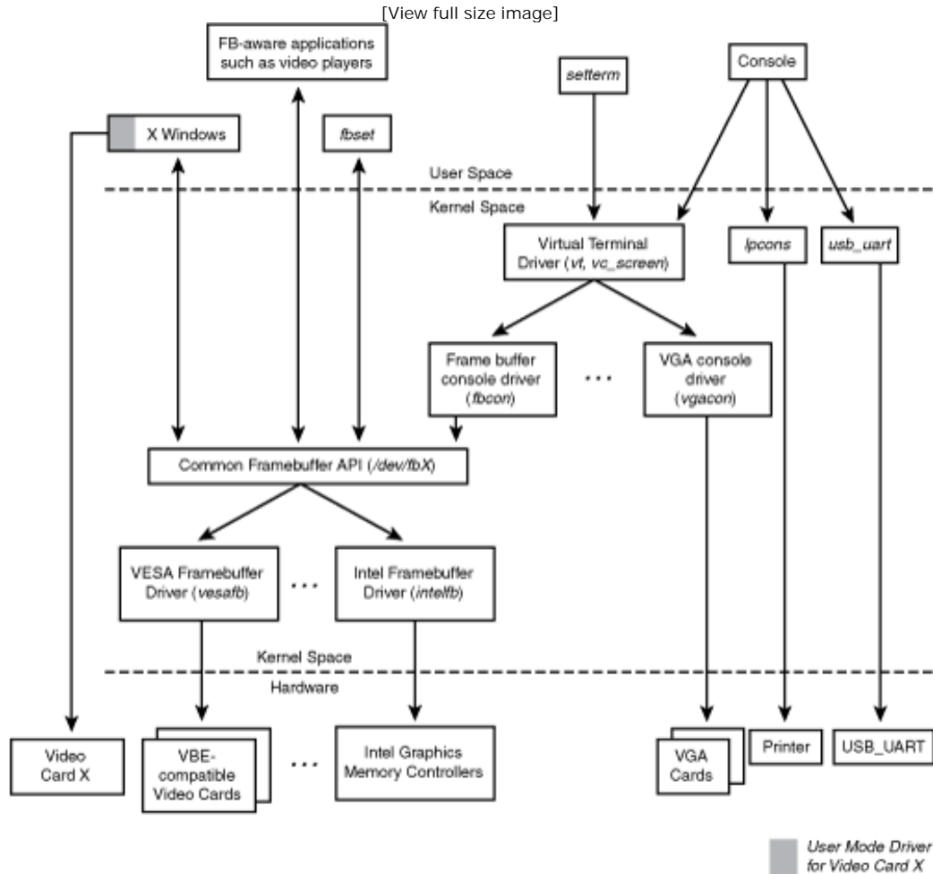
Figure 12.5. Linux-Video subsystem.
