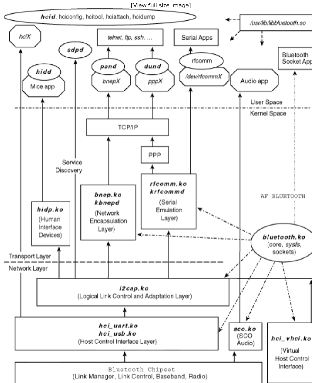
Figure 16.2. Bluetooth protocol layers mapped to BlueZ kernel modules.
