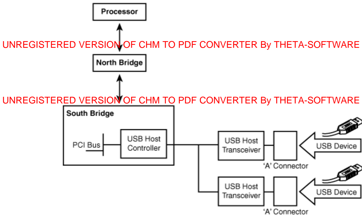
Figure 11.1. USB in the PC environment.
