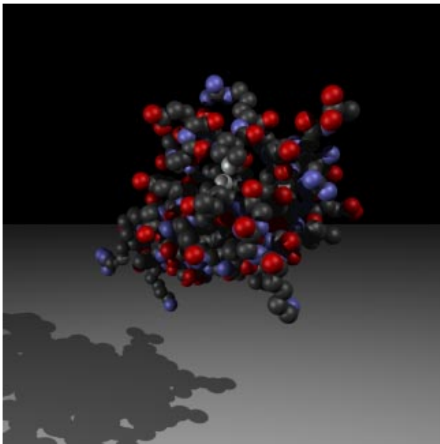
Figure 21. Molecular Visualization
