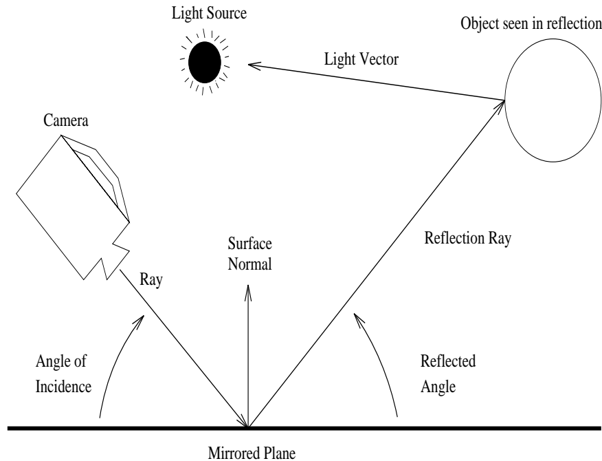
Figure 5. Specular Reflection
