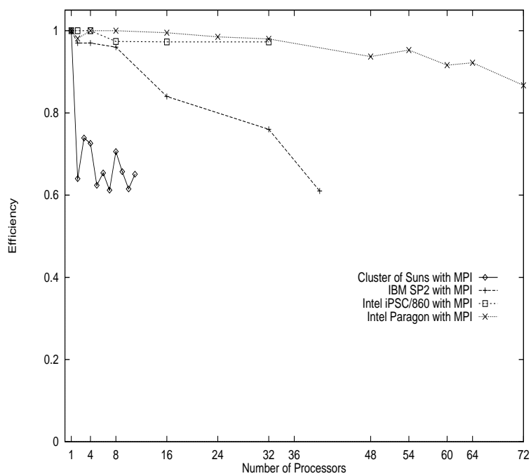
Figure 11. Plot of Efficiency for the SPD Balls Scene
