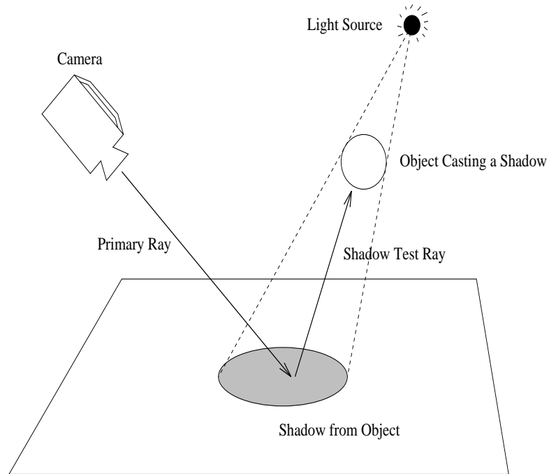
Figure 2. Shadow Cast by an Object
