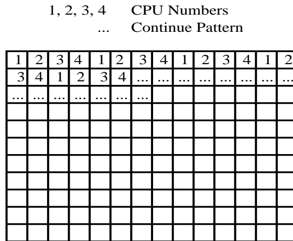
Figure 9. Pixel Cyclic Ray Tracing Decomposition
