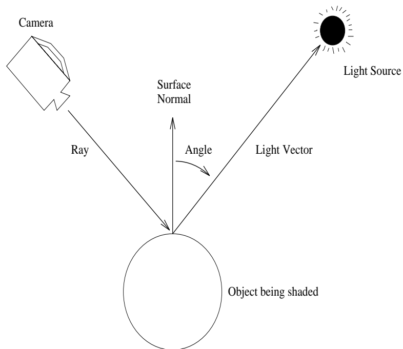
Figure 3. Diffuse Illumination of an Object
