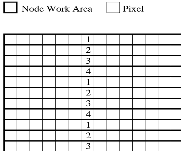
Figure 8. Scanline Cyclic Ray Tracing Decomposition
