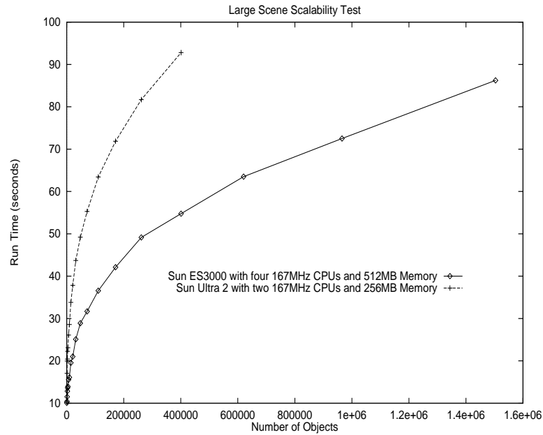
Figure 15. Large Scene Scalability Results
