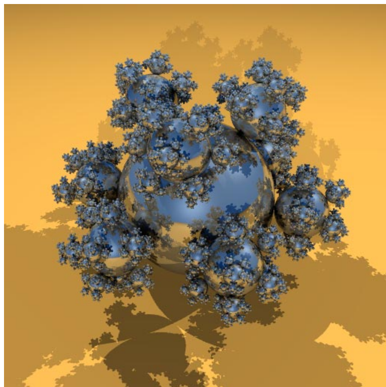
Figure 26. SPD “Sphereflake”
