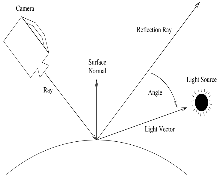
Figure 4. Phong Highlighting
