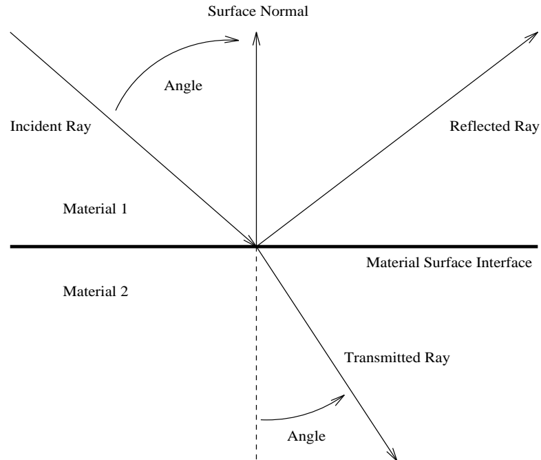
Figure 6. Refraction
