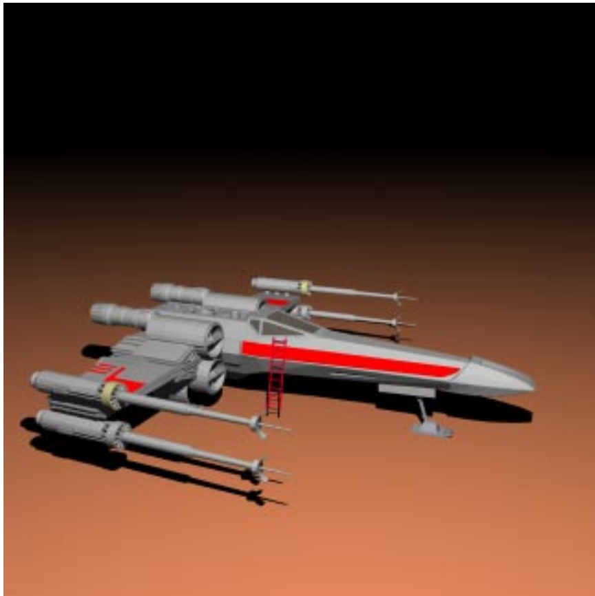
Figure 20. X-Wing Model
