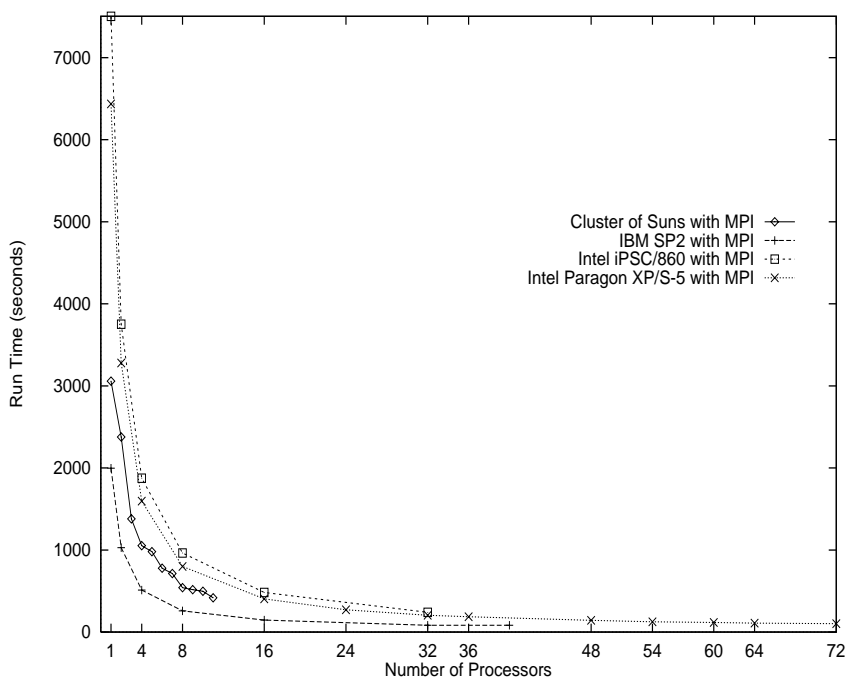
Figure 10. Plot of Execution Time for the SPD Balls Scene
